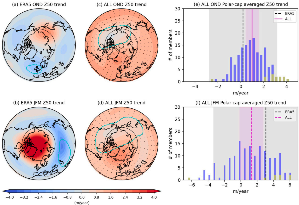
FIG. 4. As in Fig. 2, but for geopotential height at 50 hPa (Z50). It is noted that only 155 members are used in Z50 ALL MMEM. In (e) and (f), use of solid (dashed) vertical lines indicates that the trends are (are not) significant at 5% level.
