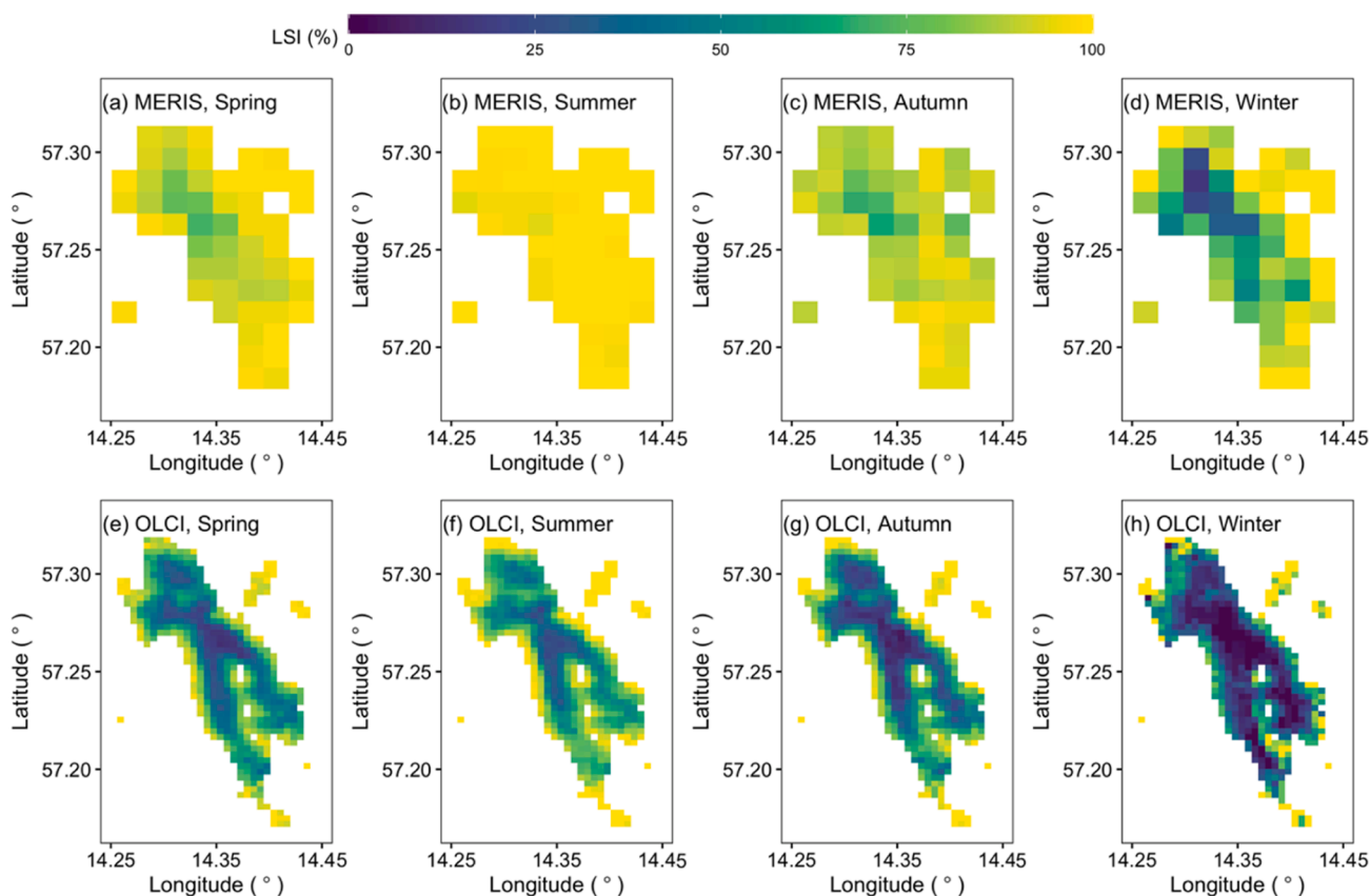
Fig. 16. Example of the seasonal variation of the frequency of observations with land-affected signals in Lake Rusken.
