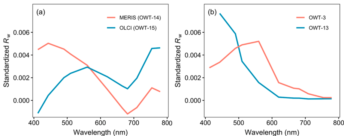
Fig. 6. (a) Typical standardized R_w spectra indicating the presence of the land-affected signal. (b) The spectral shapes of the top two dominating OWTs from Spyrakos et al. (2018) for the centres of Lakes Rusken and Bolmen.
