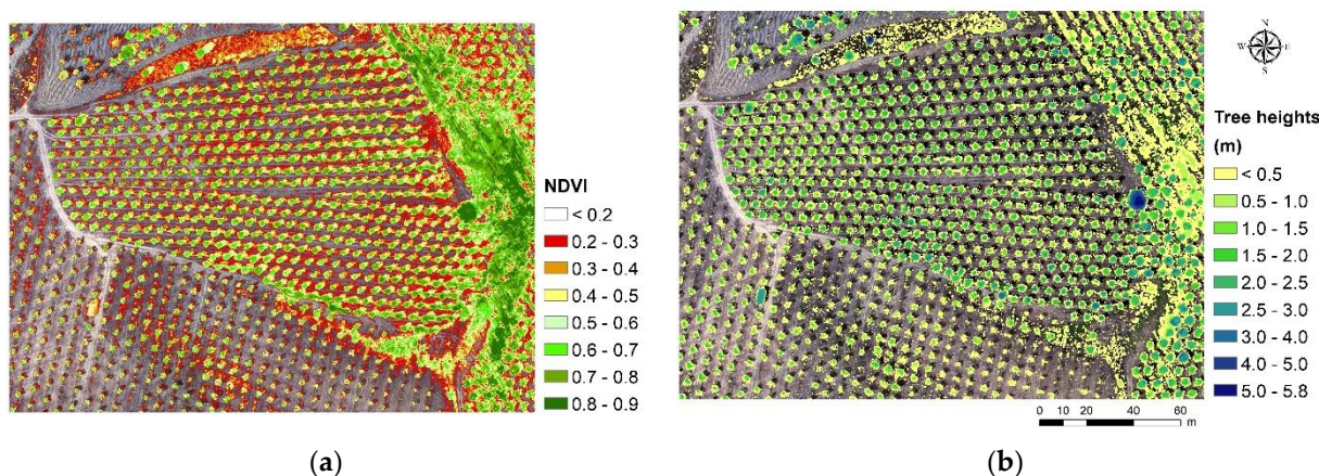
Figure 7. (a) Normalized difference vegetation index (NDVI) and (b) tree heights of an olive orchard plot ( 41^{\circ}21'31'' N, 7^{\circ}2'22'' W), derived from aerial images with the drone DJI Matrice 300 RTK using a camera RedEdge-MX (flight data: performed on 31 August 2021; 100 m altitude; 8 cm spatial resolution).
