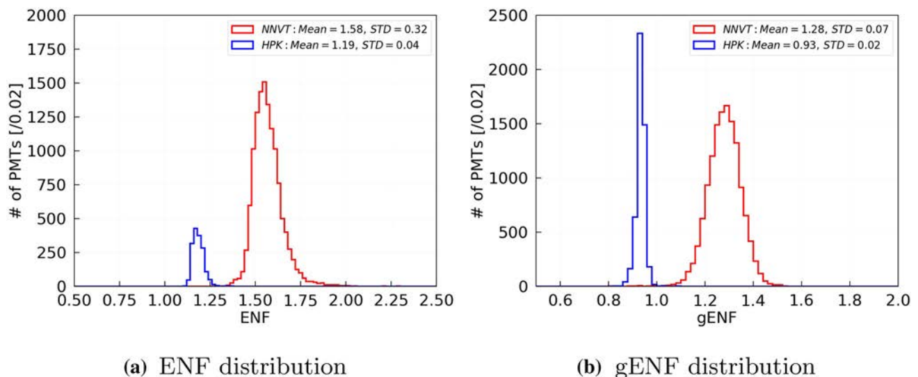
Fig. 16 Left: ENF distribution of all qualified bare PMTs. Right: gENF distribution of all qualified bare PMTs. Red: NNV; blue: HPK
