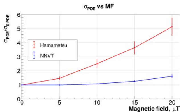
Fig. 43 PDE uniformity versus magnetic field strength. Indicated data points represent means and standard deviations of the tested samples (9 HPK PMTs and 15 NNVT PMTs)
