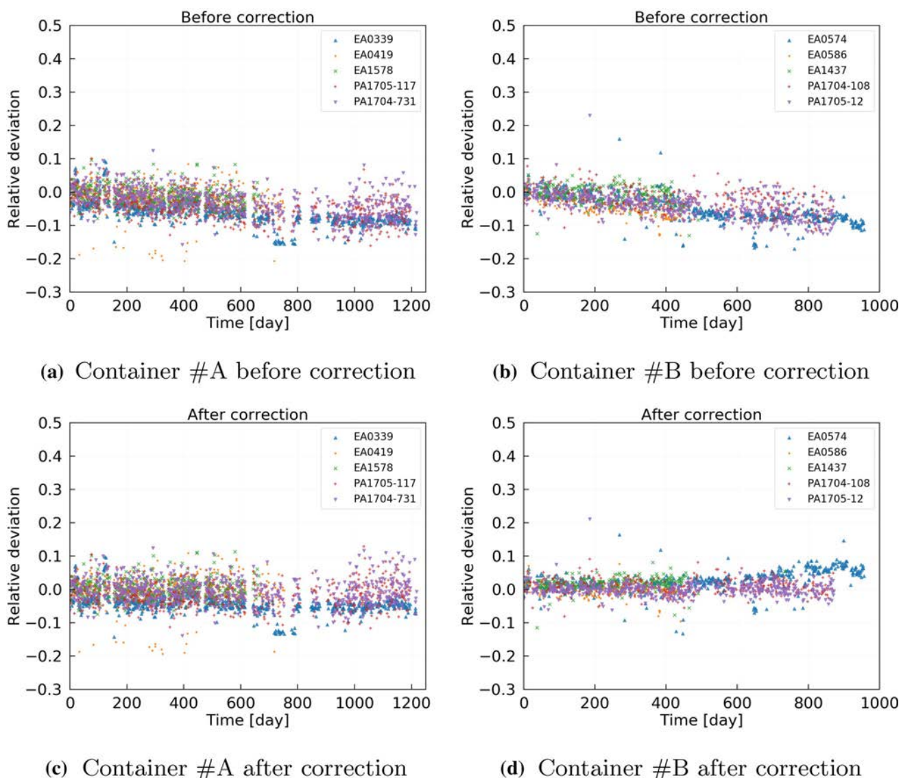
Fig. 18 Relative variation of the measured PDE of the monitoring PMTs (HPK PMTs tagged by “EA”, NNVT PMTs tagged by “PA”) at the container system, before and after a correction based on a recalibration at the end of the regular testing period. Indicated variation is
