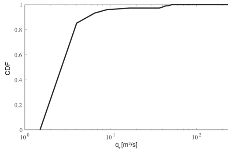
Figure 11. Cumulative distribution function (CDF) of the highest fifth percentile of the daily values of q_r at the outlet (sub10).
