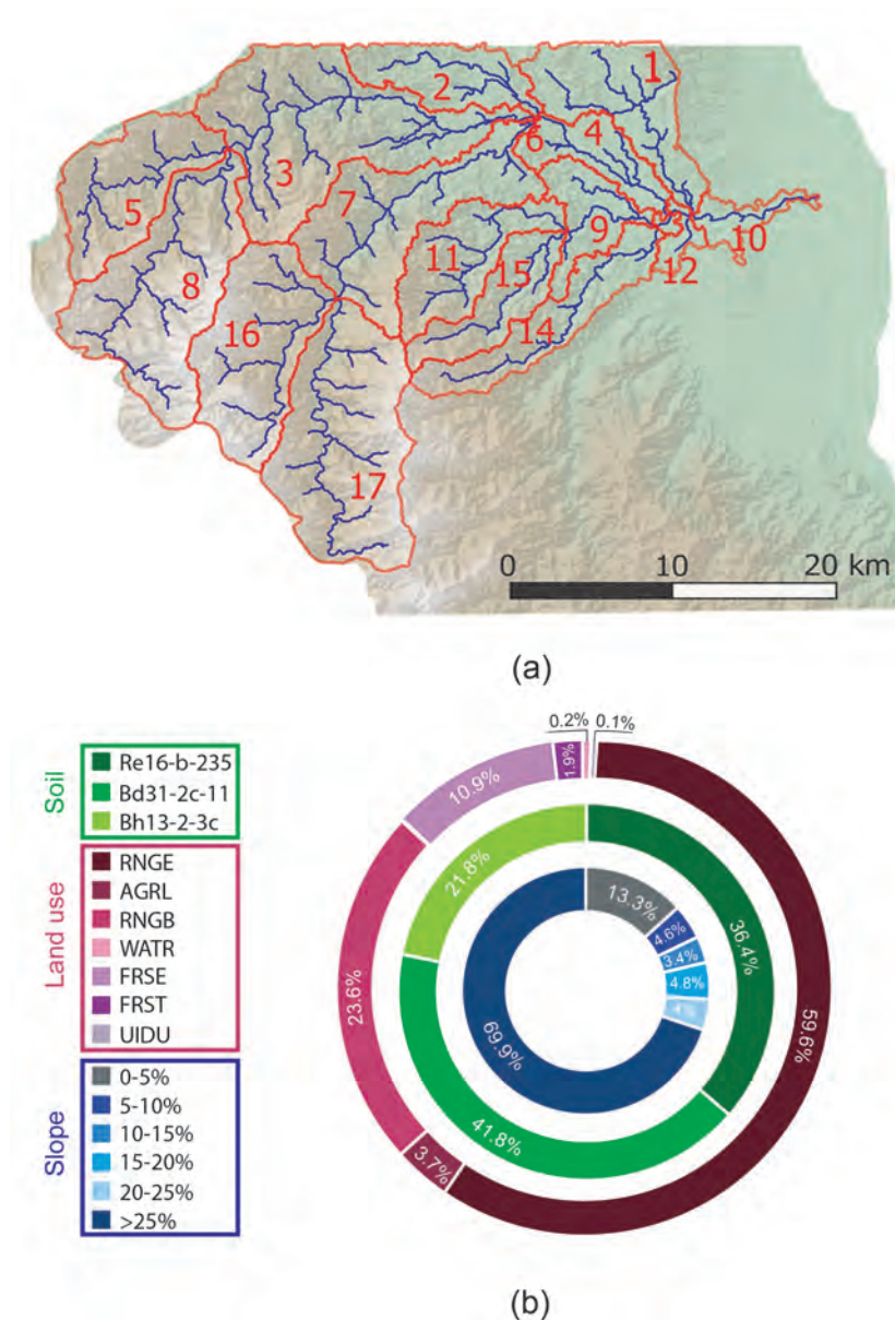
Figure 6. Delineation of the watershed and the river network (a), and percentage of the land use, soil, and slope categories across the basin (b).
