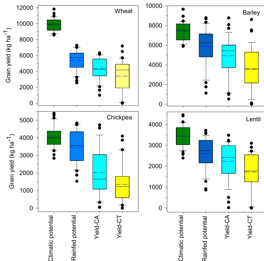
Fig. 9. Long-term (1984–2020) simulated wheat, barley, chickpea, and lentil yield ( \text{kg ha}^{-1} ) under climatic potential, rainfed potential, conservation (CA) and conventional (CT) production systems under rainfed condition in Merchouch, Morocco.
