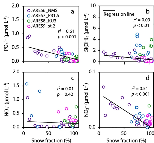
Figure 5. Plots of (a) \text{PO}_4^{3-} , (b) \text{Si}(\text{OH})_4 , (c) \text{NO}_3^- , and (d) \text{NO}_2^- concentrations for snow-origin ice versus snow fraction in multi-year ice cores.
