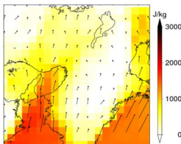
Fig. 7 Spatial distribution of CAPE (shade) and surface wind (arrows) obtained by MSM at 00:00JST on July 15 th , 2012.
