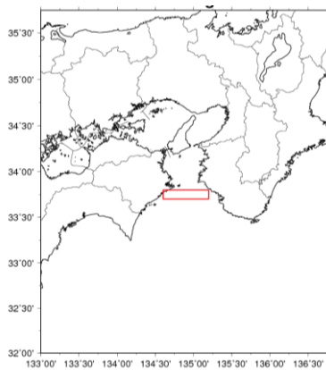
Fig. 26 Setting range for calculating the total amount of water vapor flux inflowing into the Kii channel.
