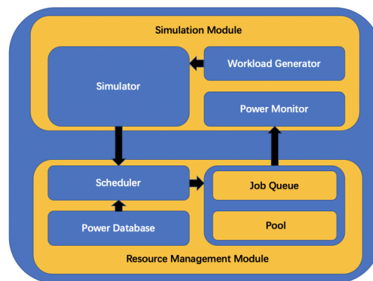
Fig. 1. Simulator architecture
