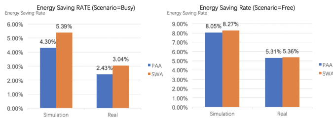
Fig. 9. Comparison of energy saving rate in multi-node situation
