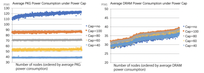
Fig. 6. Power consumption of HPCG under different power caps
