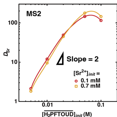
Fig. 7 Dependence of D_{Sr} on the concentration of H_2PFTOUD under H_2PFTOUD conditions ( [Sr^{2+}]_{init} is shown in the figure and [DCH18C6]_{init} = 0.02 M). The fitting curves were calculated by the least-squares method based on the extraction mechanism described by eqn (17), (18), (20), (27), (29) and (32) in text.
