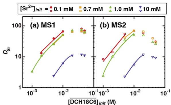
Fig. 6 Dependence of D_{Sr} on the concentrations of DCH18C6 under H_2PFTOUD conditions ( [Sr^{2+}]_{init} and [DCH18C6]_{init} are shown in the figure and [H_2PFTOUD]_{init} = 0.02 M). The solid lines are fitting curves based on the extraction mechanism described by eqn (17), (18), (20), (27), (29) and (32) in text.
