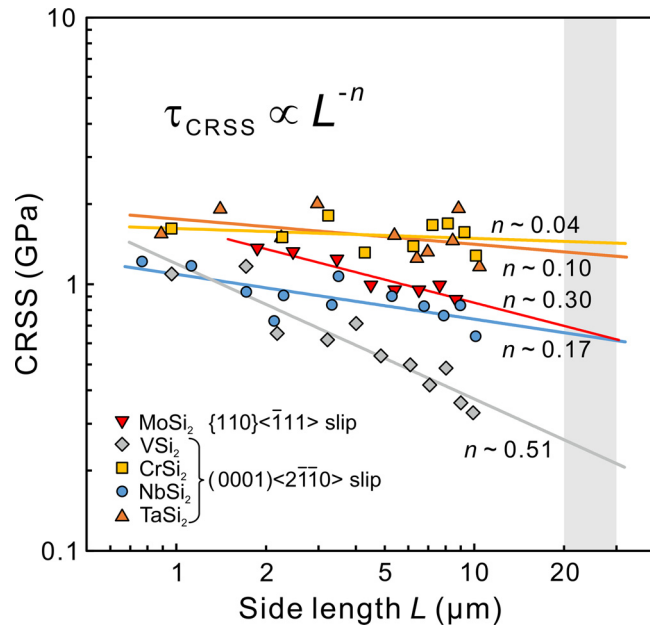
Fig. 8. (a) Specimen size dependence of CRSS for \{110\}\langle\bar{1}11\rangle slip in \text{C11}_b - \text{MoSi}_2 and \{0001\}[2\bar{1}10] slip in \text{C40} - \text{VSi}_2 , \text{CrSi}_2 , \text{NbSi}_2 and \text{TaSi}_2 .
