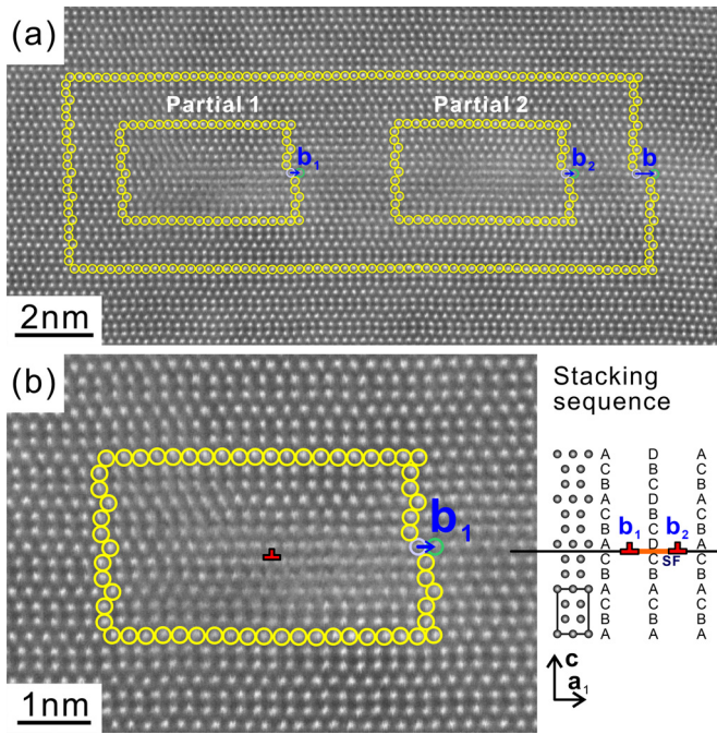
Fig. 7. (a) HAADF-STEM image of core structure of a 1/3[2\bar{1}10] edge dislocation introduced in 2\bar{1}1\bar{2} -oriented micropillar of \text{NbSi}_2 with L = 7.9 \mu\text{m} . (b) High-magnification image of core structure of the partial dislocation 1 in (a). The results of analysis of stacking order in the fault region between two partials are indicated in the bottom right.
