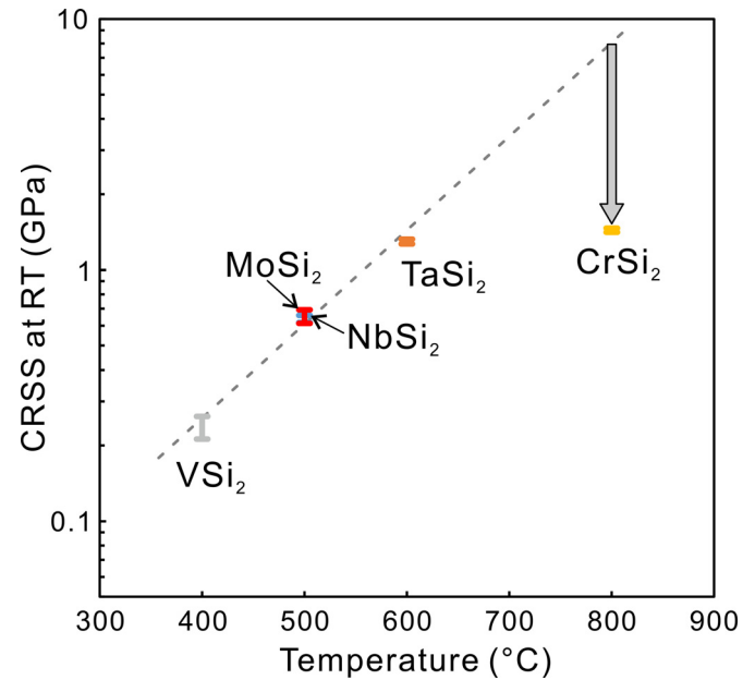
Fig. 9. Relationship between the extrapolated bulk CRSS values obtained from micropillar compression tests for \text{C11}_b and \text{C40} TM disilicides and the onset temperature for plastic flow of the corresponding bulk single crystals by the operation of their equivalent slip systems.
