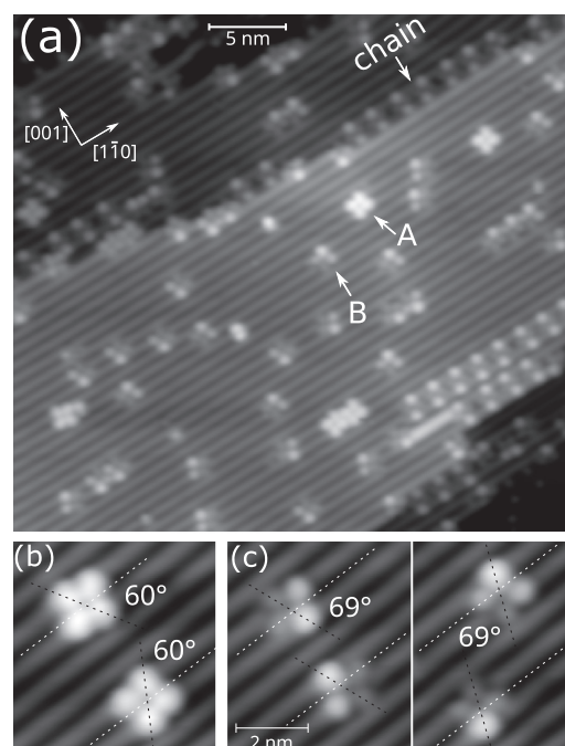
Figure 1: (a) Typical STM image of the Au(110)-( 1 \times 2 ) surface under initial exposure to CuPc vapor. The straight lines along [1\bar{1}0] are the missing rows of Au. Two types of monomers (denoted as A and B ) and CuPc chains are observed. (b) Two equivalent orientations of A -CuPc. (c) Four orientations of B -CuPc. The angles between [1\bar{1}0] and the diagonal line of CuPc were 60^\circ and 69^\circ for A -CuPc and B -CuPc, respectively. The images were obtained at V_s = 200 mV and I = 1 nA.
