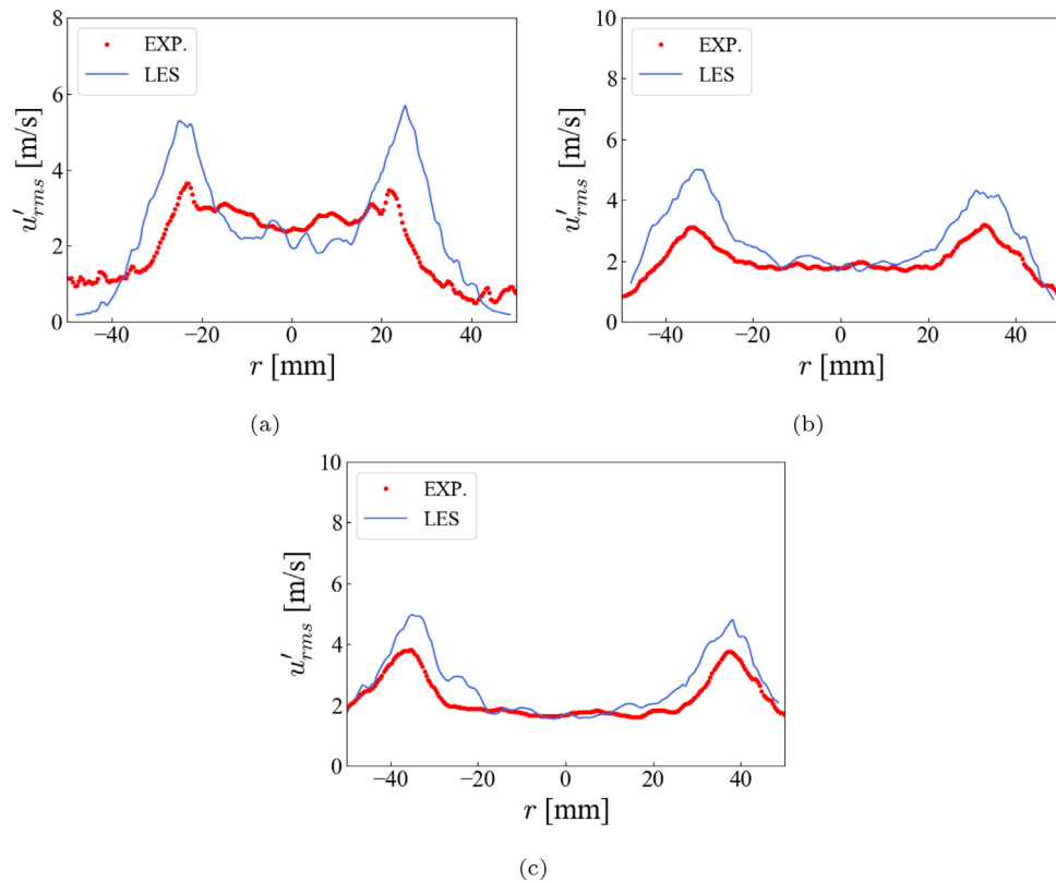
Fig. 12. Comparisons of radial profiles of RMS of axial velocity fluctuations between experimental data and LES predictions at different stream-wise locations of (a) x = 17.5 mm, (b) x = 35 mm and (c) x = 52.5 mm.
