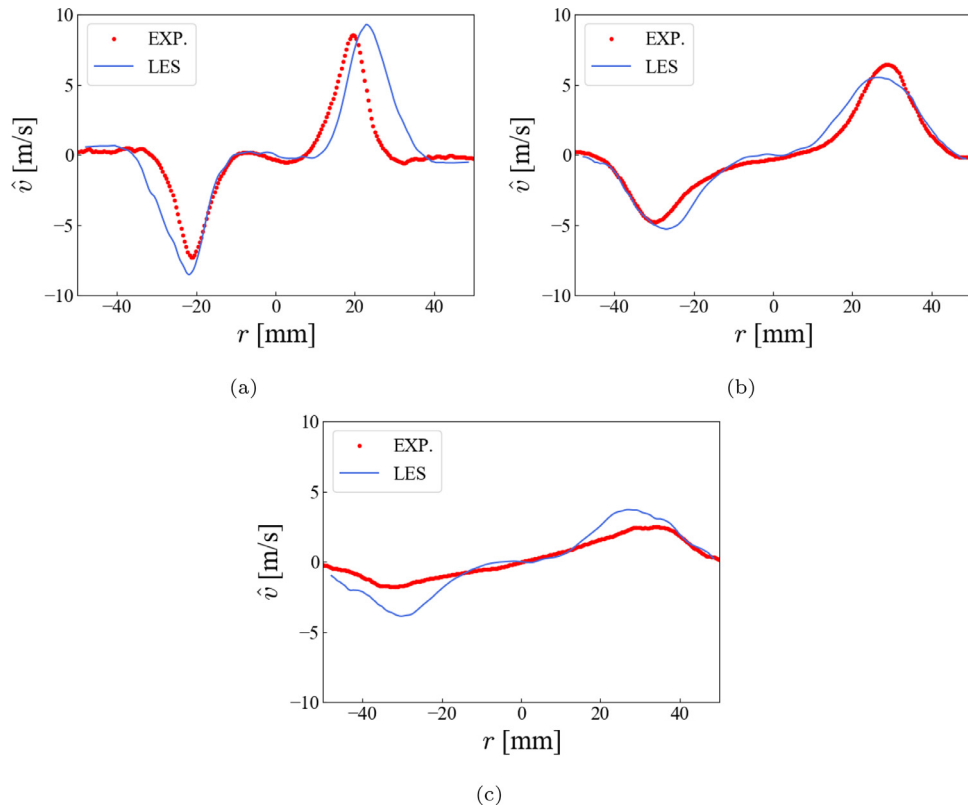
Fig. 11. Comparisons of radial profiles of time-averaged radial velocity between experimental data and LES predictions at different stream-wise locations of (a) x = 17.5 mm, (b) x = 35 mm and (c) x = 52.5 mm.
