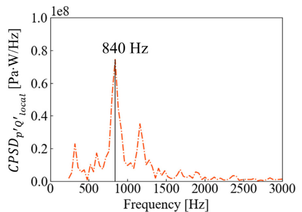
Fig. 26. Cross power spectral density CPSP_{p'Q'_{local}} between the acoustic pressure perturbations p' computed at (x, y) = (50 mm, 180 mm), and the local heat release rate fluctuation Q'_{local} occurring in the region indicated by the yellow square in Fig. 24.
