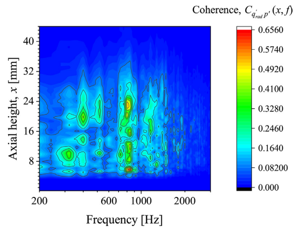
Fig. 23. Stream-wise variation of the spectrum of coherence C_{q'_{rad} p'}(x, f) between the radially integrated heat release rate fluctuations q'_{rad}(x) and the far-field acoustic pressure perturbations p' sampled at (x, y) = (50 \text{ mm}, 180 \text{ mm}) .
