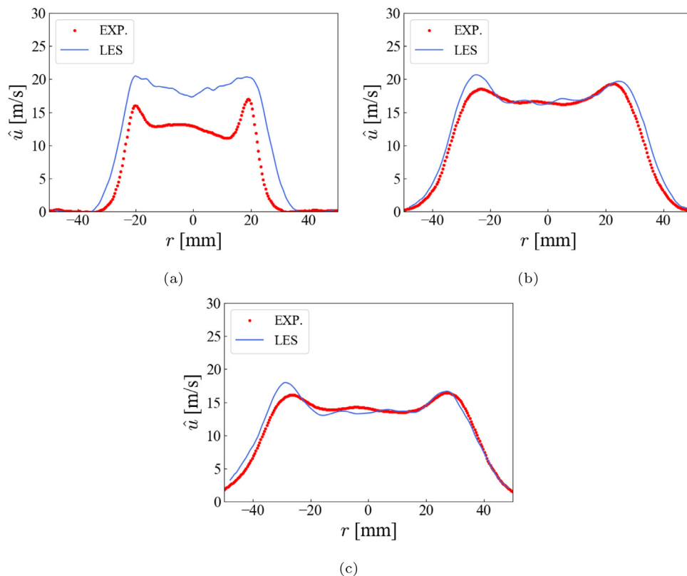
Fig. 10. Comparisons of radial profiles of time-averaged axial velocity between experimental data and LES predictions at different stream-wise locations of (a) x = 17.5 mm, (b) x = 35 mm and (c) x = 52.5 mm.
