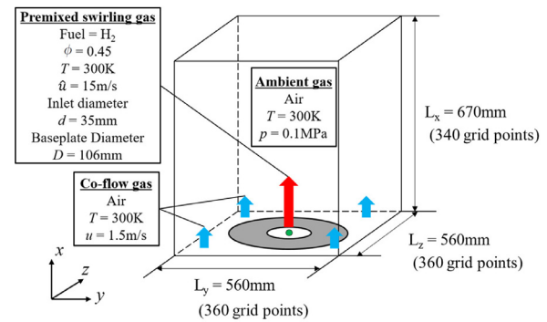
Fig. 3. Schematic of computational domain and conditions for LES.
