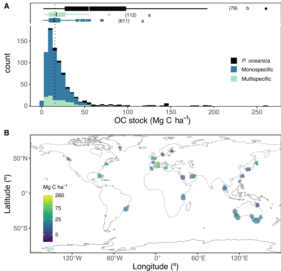
Figure 2. Influence of meadow type on organic carbon (OC) stocks and global map of OC stocks “hotspots.” (a) Histogram showing the distribution of OC stocks for each type of meadow considered by our model ( Posidonia oceanica , monospecific, and multispecific). Note that the distribution of P. oceanica OC stocks is extremely skewed to the right, compared to the rest of monospecific and mixed meadows. Overlaid on the histogram, boxplots for each meadow type support model results, with P. oceanica meadows having higher OC stocks than the rest of monospecific and mixed meadows. Dotted vertical line illustrates the global median considering all samples together. Different lower-case letters next to each box correspond to Tukey Honestly Significant Difference post-hoc tests with p -value < 0.05. Number of cores for each group are given in brackets. (b) Geographical distribution of seagrass soil sections compiled in this study colored according to their OC stocks. The Mediterranean appears as the clearest hotspot of OC stocks, coherent with P. oceanica (endemic to the Mediterranean) being the seagrass with highest OC stocks. Note that points have some transparency, thus, the more solid the point looks, the greater the density of samples. Note that points have been jittered for improved visualization, as well.
