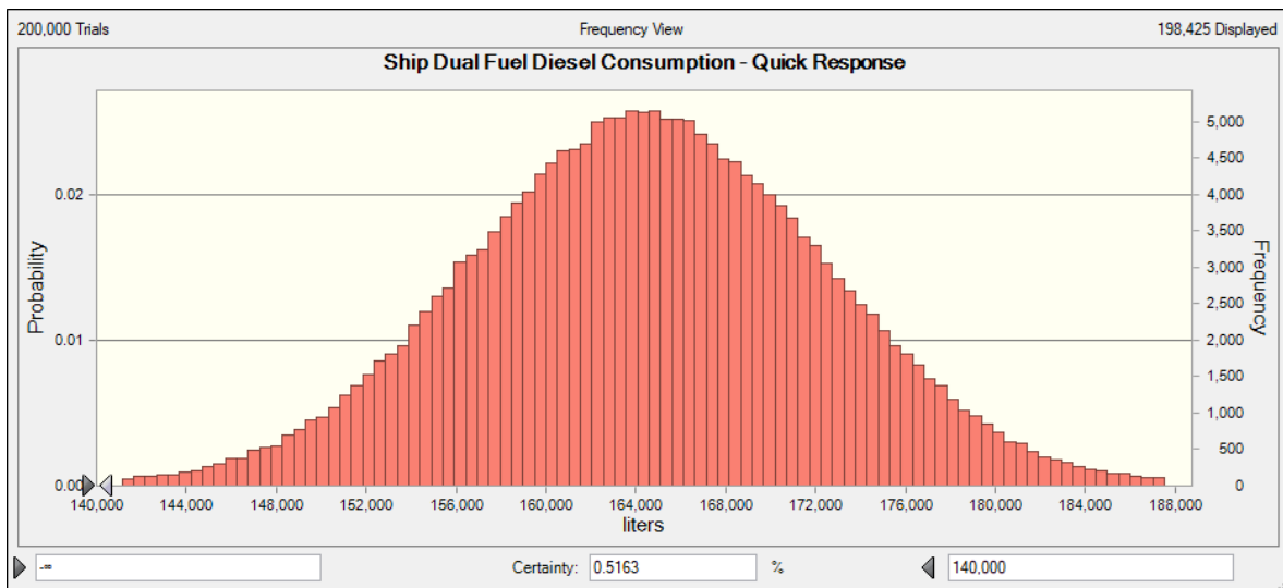
Figure 8. Diesel consumption during a quick response mission (dual fuel).
