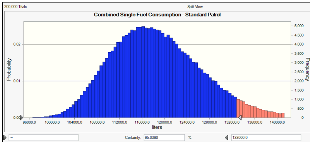
Figure 7. JP-5 consumption during standard patrol mission (SFC).
