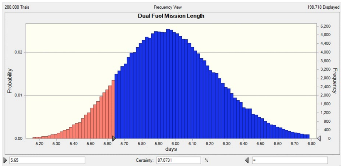
Figure 12. Length of the operation for a quick response mission (status quo – dual fuel).
