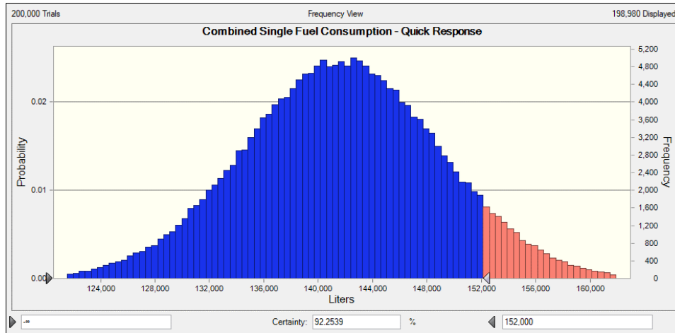
Figure 15. JP-5 combined consumption during a 5.65-day quick response mission (SFC).
