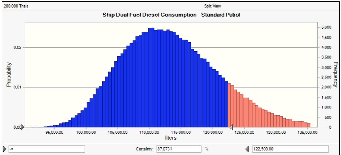
Figure 5. Diesel consumption during standard patrol mission (status quo).
