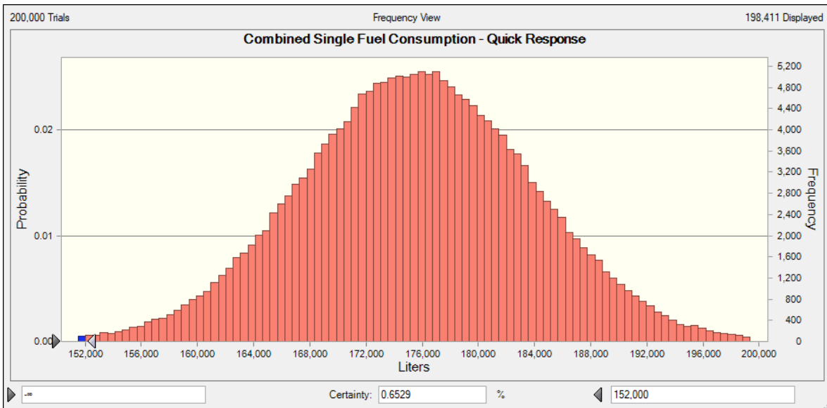
Figure 10. JP-5 consumption during a quick response mission (SFC).
