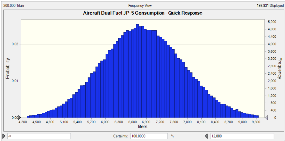
Figure 9. JP-5 consumption during quick response mission (status quo).
