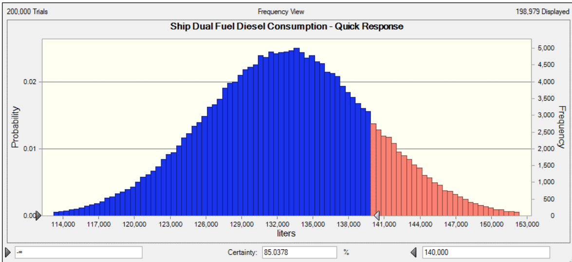
Figure 13. Diesel consumption during a 5.65-day quick response mission (status quo).
