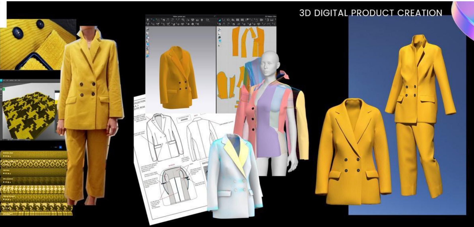
Material Digitization
