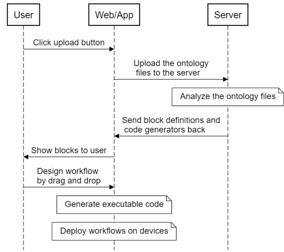
Fig. 2. A time sequence diagram of user interactions and the subsequent system processes.
