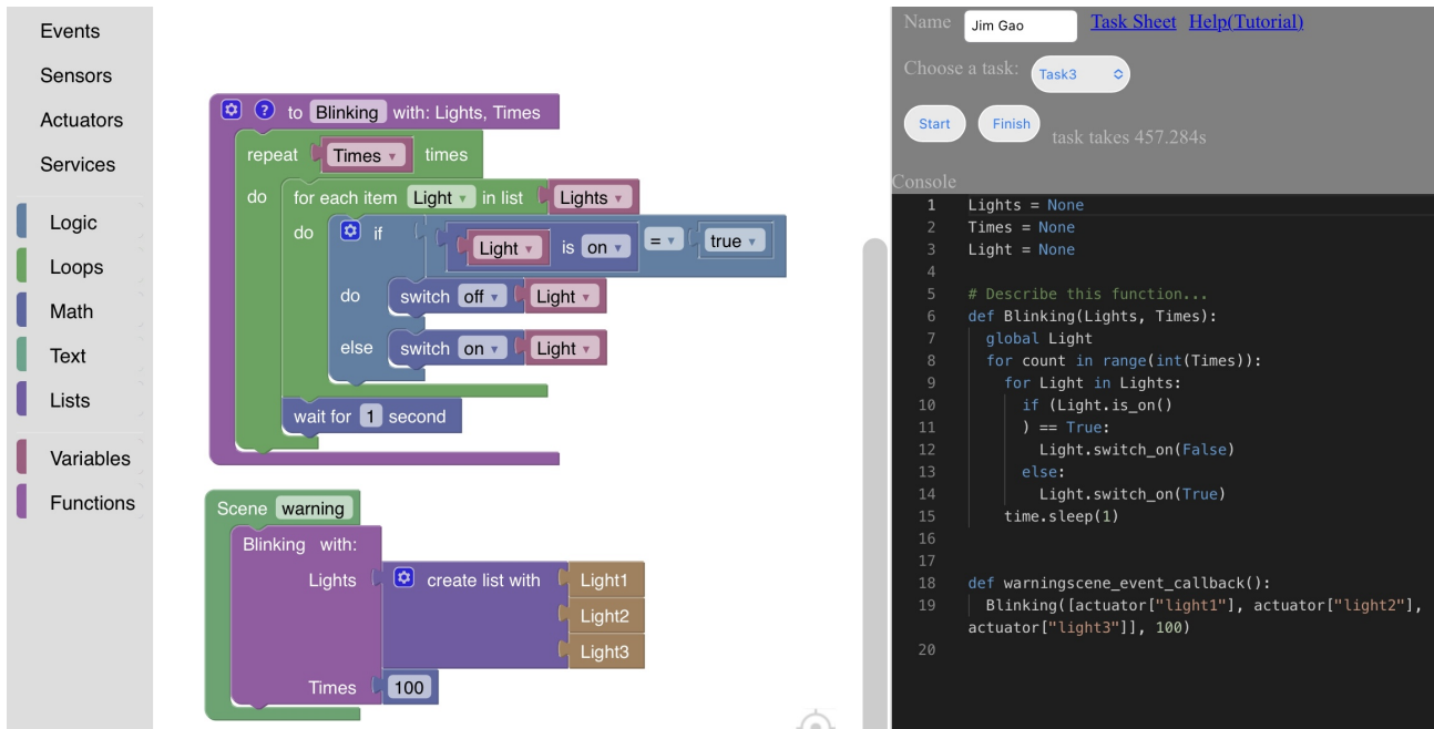
Fig. 3. The interface of the web-based HolonCraft client application.
