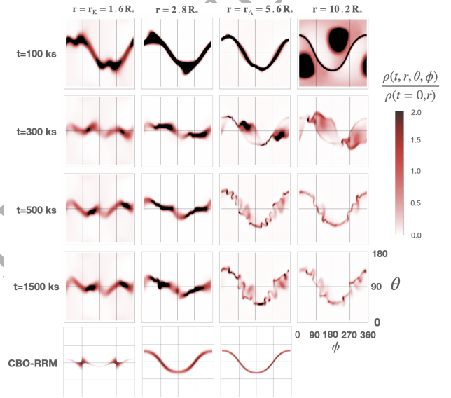
Figure 9. For tilted dipole \beta = 45^\circ , radial slices of density plotted as a function of azimuth and co-latitude at the various radii labeled at the top, with time progression of MHD model in four rows at labeled time snapshots. The bottom row shows for comparison the corresponding density distribution of the CBO-RRM model.
