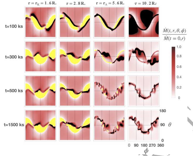
Figure 8. For tilted dipole \beta = 45^\circ , mass flux plotted as a function of the azimuth and co-latitude at various radii. The columns show slices at the 4 labeled radii, while rows show snapshots at the 4 labeled times. Yellow denotes regions of infall.
