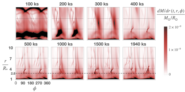
Figure 7. For MHD simulation of tilted dipole \beta = 45^\circ , time evolution of the latitudinally averaged mass distribution in radius dM/dr , plotted versus radius and azimuth. After about 500 ks, the model reaches a quasi-steady state with episodic mass ejections distributed about the y-axis ( \phi = 90^\circ and \phi = 270^\circ ), where the magnetic and rotational equatorial planes intersect. The horizontal dotted line at r = 2.8R_* marks the boundary between magnetically confined material, and the onset of CBO events.
