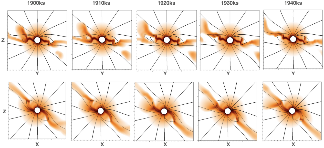
Figure 5. Time evolution over the last five snapshots ( t = 1900 - 1940 ks) of log density and field lines, showing both yz (top) and xz (bottom) slices, now extending over spatial range of \pm 10R_* . In the yz cut note the progressive field line stretching and mass ejection associated with a centrifugal breakout event. Breakouts also occur in the xz cut but they are more conspicuous in a different snapshot due to slight left-right asymmetry in the numerical model. Evidence of such breakout events are quite apparent in figure 7 as well and occur on about 50 ks timescale .
