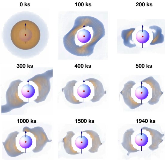
Figure 1. Time evolution of the standard model ( \eta_* = 10^3 , W = 1/2 , \beta = 45^\circ ), showing volume renderings of the density structure as viewed from the rotational pole (red dot), with projected magnetic axis (blue arrow) directed upward. After initial transients, the dragonfly wing-like co-rotating structure settles into a quasi-steady state with occasional outbreaks due to centrifugal forces. .
