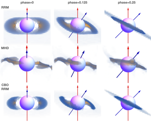
Figure 6. For standard oblique dipole case ( \beta = 45^\circ and W = 0.5 ), comparison of the phase variation of volume-rendered density for the final time ( t = 1940 ks) of the MHD simulation (center row) with predictions of the analytic Rigidly Rotating Magnetosphere (RRM) model. The top row depicts the density distribution resulting from wind feeding over a fixed time, as assumed in the original RRM analysis of Townsend & Owocki (2005). The bottom row shows a modified scaling to mimic predictions of a centrifugal breakout (CBO) analysis, with higher concentration along the common magnetic-rotational equator (y-axis) and a radial decline in surface density, \sigma \sim 1/r^5 , that is steeper than the \sigma \sim 1/r^3 for fixed-time wind-feeding along a dipole field. The blue vectors depict the magnetic dipole axis, and the observer inclination is i = 90^\circ , and so perpendicular to the red vectors representing the fixed stellar rotation axis.
