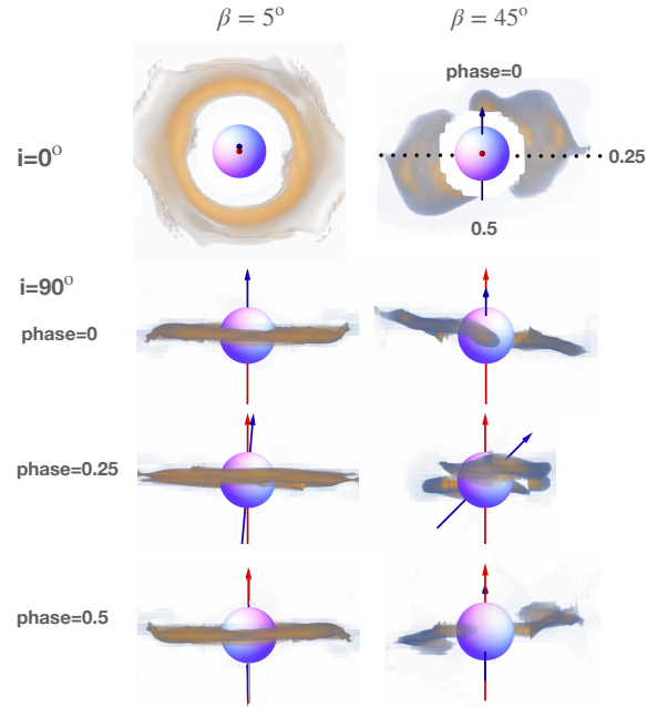
Figure 2. As in figure 1, volume renderings of density structure, now comparing representative evolved time step ( t = 1000 ks) structures of two different models with identical magnetic field, rotation but different obliquity, \beta : 45^\circ (right) and 5^\circ (left). Notice how higher obliquity model restricts density in the azimuthal direction. This is a result of complex dynamics between rotation and strong tilted magnetic field.
