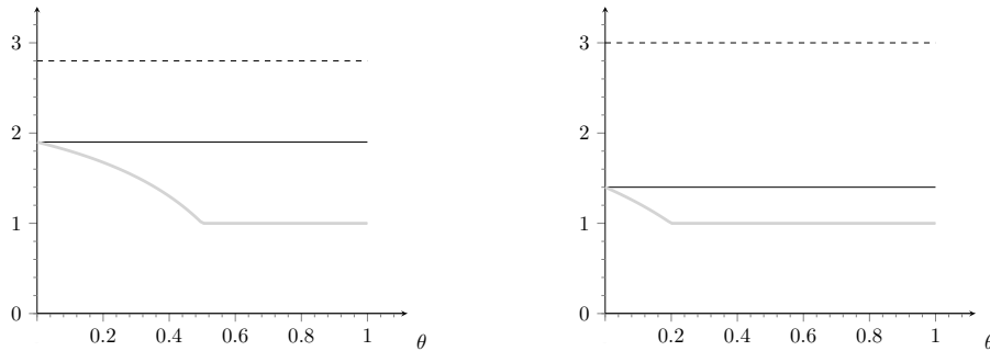
Figure 3: Left: a Kleinian limit set with \delta = 1.9 and k_{\min} = k_{\max} = 1 . Right: a Julia set with h = 1.4 and p_{\max} = 4 .
