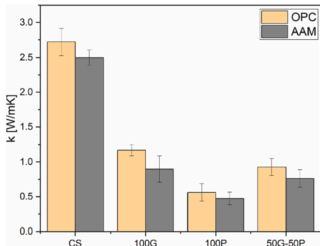
Fig. 10. Thermal conductivity of the composites.
