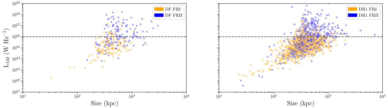
Figure 3. Luminosity versus size distribution of the FRI (yellow circles) and FRIIs (blue squares) for the combined deep fields (left) and the LoTSS-DR1 sources from M19 (right). The dashed line shows the ‘traditional’ boundary between FRI and FRII, at L_{150} \sim 10^{26} \text{ W Hz}^{-1} (Fanaroff & Riley 1974; Ledlow & Owen 1996).
