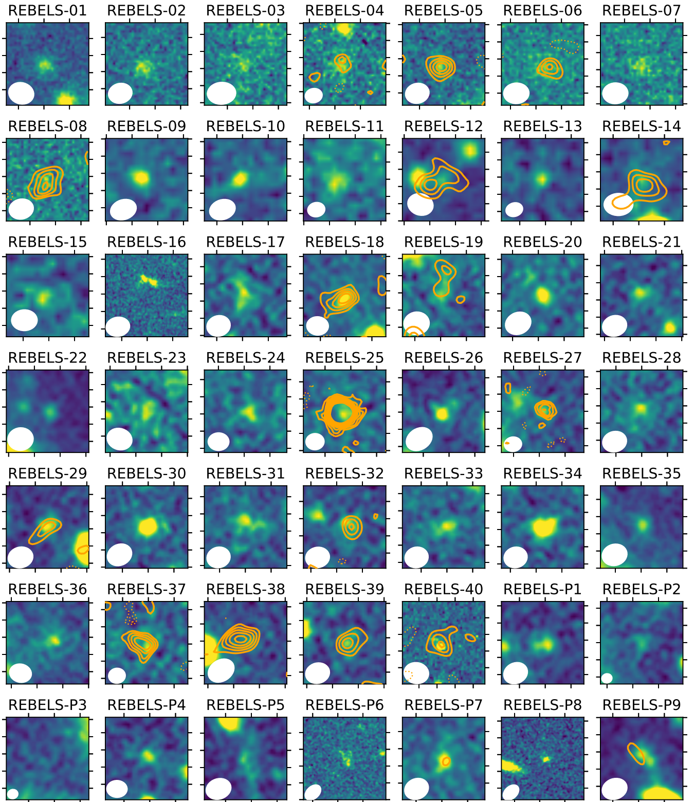
Figure A1. The same as Figure 3 without the [C II] contours. The targets without a dust continuum detection are also shown.
