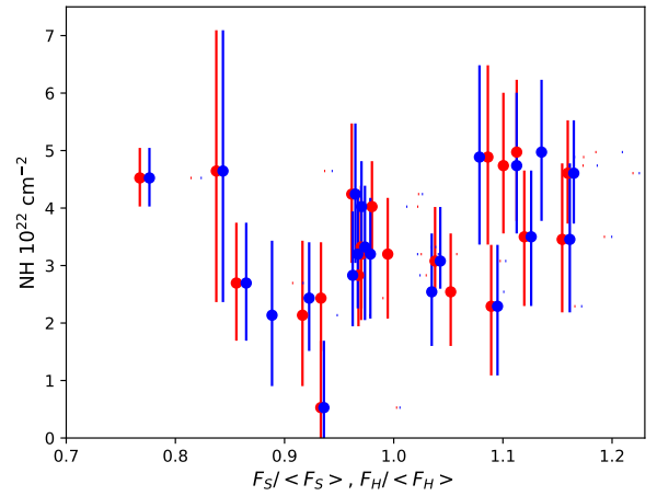
Fig. 12. Best-fit values of N_{\text{H}} plotted against the ratio of the flux in each Obsid over the average flux (red and blue dots correspond to the soft and hard bands, respectively).
