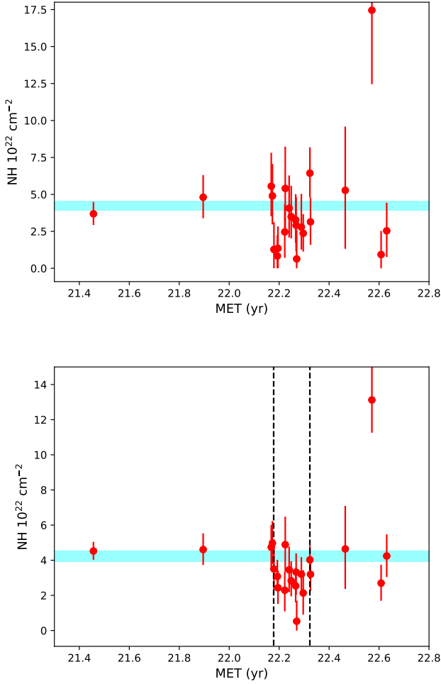
Fig. 10. Upper panel: best-fit values of N_{\text{H}} for each Obsid as a function of the Mission Timeline MET (years). The first point has been moved to 21.5 to be shown in the same linear plot. The horizontal shaded line shows the best-fit value of the cumulative spectrum with PSF correction, as listed in Table 1. Lower panel: same, but with best-fit values of N_{\text{H}} obtained with \Gamma frozen to 1.88. The vertical dashed lines bracket the period with low intrinsic absorption as discussed in the text.
