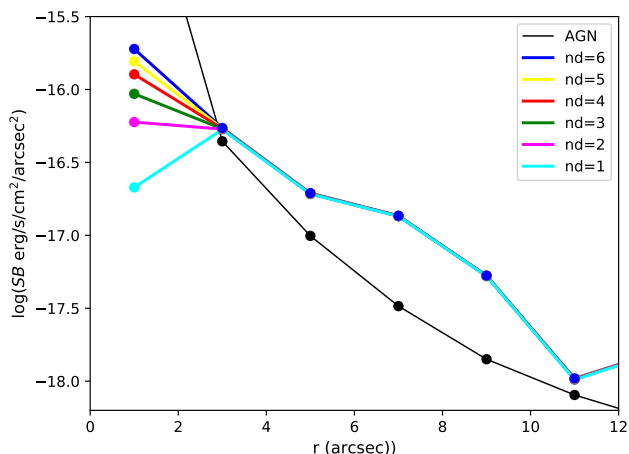
Fig. 5. Azimuthally averaged profile of the diffuse emission (after subtraction of the AGN emission and of the background) at different n_d values. As expected, only the innermost bin is affected by the choice of n_d , while the indirect effects on the normalization of the AGN contamination, thus on the overall normalization of the diffuse emission, is negligible. The black line is the simulated AGN emission for comparison.
