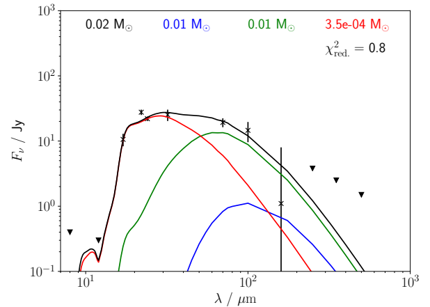
Figure 5. Cas A post-shock dust SED (black crosses) and best-fit model SEDs for clumped 0.1 \mu\text{m} (blue), clumped 5 \text{ nm} (green), and diffuse 0.1 \mu\text{m} (red) grains, with the total model SED shown in black.
