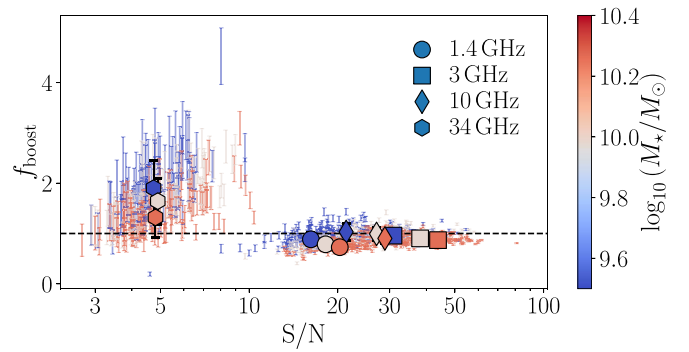
Figure 12. Median boosting as a function of S/N for stacks of simulated sources drawn from the bins defined in Table 2. Points are colored by their stellar mass—at fixed redshift, lower-mass galaxies are typically fainter, and hence will show a greater level of median boosting. The correction factor is around unity at 1.4, 3, and 10 GHz, but reaches f_{\text{boost}} = 1.9 ( \sigma = 0.5 ) for the low-mass bin at 34 GHz. All median-stacked flux densities presented in this work are corrected for boosting.
