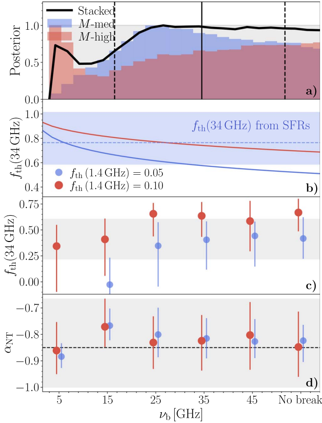
Figure 9. A quantitative test of synchrotron aging in the radio spectra of typical high-redshift star-forming galaxies. (a) Posterior distributions of the break frequency \nu'_b in bins M -med and M -high, obtained after explicitly including a spectral break in the fitting. The combined posterior is shown through the solid black line, while the prior is shown through the gray rectangle. The solid and dashed vertical lines indicate the median and 16–84th percentiles from the combined posterior, respectively. High break frequencies \nu'_b \gtrsim 15 GHz are favored by the fitting routine. (b) The 34 GHz thermal fraction as a function of \nu'_b for an M82-like spectrum at z = 1 , given a 1.4 GHz thermal fraction of 10% (as in M82; red line) and 5% (as in Murphy 2013; blue line). The shaded blue region shows the expected thermal fraction based on the stacked synchrotron SFRs. A 5% thermal fraction at 1.4 GHz requires the existence of a low-frequency break ( \nu'_b \lesssim 25 GHz) in order to match the measured f_{\text{th}}(34 \text{ GHz}) . This, however, is disfavored by the posterior in panel (a). (c) and (d) Illustration of the biases induced when fitting complex spectra with a simple model. The recovered thermal fractions (c) and synchrotron spectral indices (d), obtained from fitting simulated radio spectra, are shown as a function of break frequency. The colored points indicate the median recovered value among the simulations, given an input thermal fraction at rest-frame 1.4 GHz, and the 16–84 percentile spread. The gray bands indicate the observed range of 34 GHz thermal fractions and synchrotron slopes when fitting the combined COSMOS and GOODS-N stacks with our model in Equation (4). A break in the radio spectrum is plausible when the observed and simulated spread among both f_{\text{th}} and \alpha_{\text{NT}} are similar, though the latter parameter does not provide meaningful constraints. A combination of either f_{\text{th}}(1.4 \text{ GHz}) = 0.05 and \nu'_b \gtrsim 30 GHz or f_{\text{th}}(1.4 \text{ GHz}) = 0.10 and 15 \text{ GHz} \lesssim \nu'_b \lesssim 25 GHz provides a reasonable match between simulations and observations. Upon combining the constraints across the four panels, we qualitatively infer that the radio spectrum of star-forming galaxies can be characterized by a typical thermal fraction ( f_{\text{th}}(1.4 \text{ GHz}) \sim 0.10 ) and a spectral break at \nu'_b \sim 15 –25 GHz.
