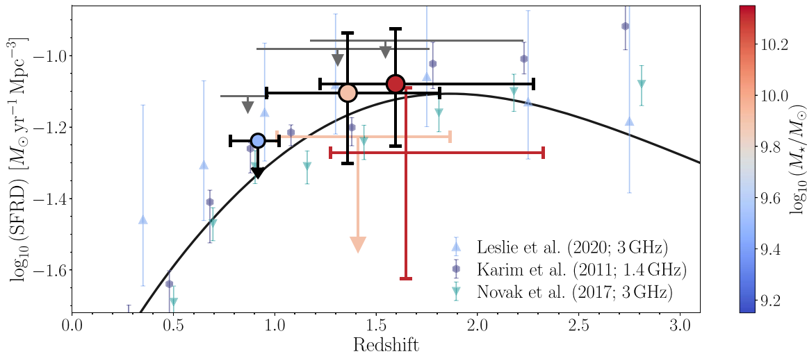
Figure 11. Constraints on the cosmic star formation history from free–free emission. The large points, placed at the median redshift of the corresponding bin, present the most robust constraints and adopt a thermal fraction f_{\text{th}}(34 \text{ GHz}) = 0.77^{+0.25}_{-0.18} , as determined through a comparison of synchrotron and free–free SFRs (case 3; Section 5.1). Upper limits, assuming a thermal fraction of unity, are shown via gray arrows (case 2). The colored error bars show the cosmic star formation rate density when the fitted thermal fractions are adopted for the two bins with a stacked detection at 34 GHz (case 1; fits do not include a spectral break). The horizontal error bars show the interquartile ranges for the corresponding redshift bins. The canonical Madau & Dickinson (2014) cosmic SFRD is shown through the black curve, and various radio-based studies, using nonthermal synchrotron emission as a star formation tracer, are additionally overplotted. Similar to this work, Karim et al. (2011) and Leslie et al. (2020) utilize a radio stacking analysis at low frequencies (1.4 and 3 GHz, respectively), while Novak et al. (2017) use radio-detected sources. Our constraints are in good agreement with those from commonly adopted star formation tracers at high redshift and show that radio free–free emission can be used to constrain cosmic star formation.
