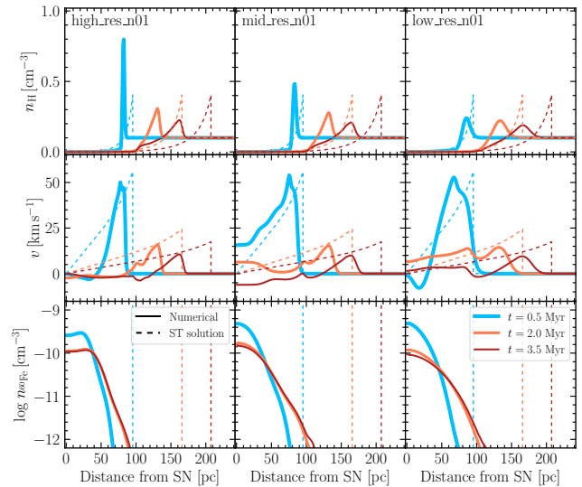
Figure A1. Convergence with gas-particle mass. The resolution increases from right to left. Shown are the average radial profiles of hydrogen number density ( top ), gas radial velocity ( middle ), and number density of ^{60}\text{Fe} ( bottom ) in the simulations with gas-particle mass M_{\text{gas}} = 3 \times 10^{-2} M_{\odot} ( high_res_n01 , left ), M_{\text{gas}} = 24 \times 10^{-2} M_{\odot} ( middle_res_n01 , middle ), and M_{\text{gas}} = 192 \times 10^{-2} M_{\odot} ( low_res_n01 , right ). The profiles are displayed at three consecutive times: 0.5 Myr (light-blue), 2.0 Myr (orange), and 3.5 Myr (dark-red) Myr. The mean ISM density is n_{\text{H}} = 0.1 \text{ cm}^{-3} in all cases. The width of radial bins is 1 pc. For reference, we use the thin dashed curves to indicate the ideal density profiles ( top ), velocity profiles ( middle ) and forward shock positions ( bottom ) in the ST solution. To compute the ejecta density we assumed M_{60\text{Fe,tot}} = 10^{-4} M_{\odot} and no radioactive decay.
