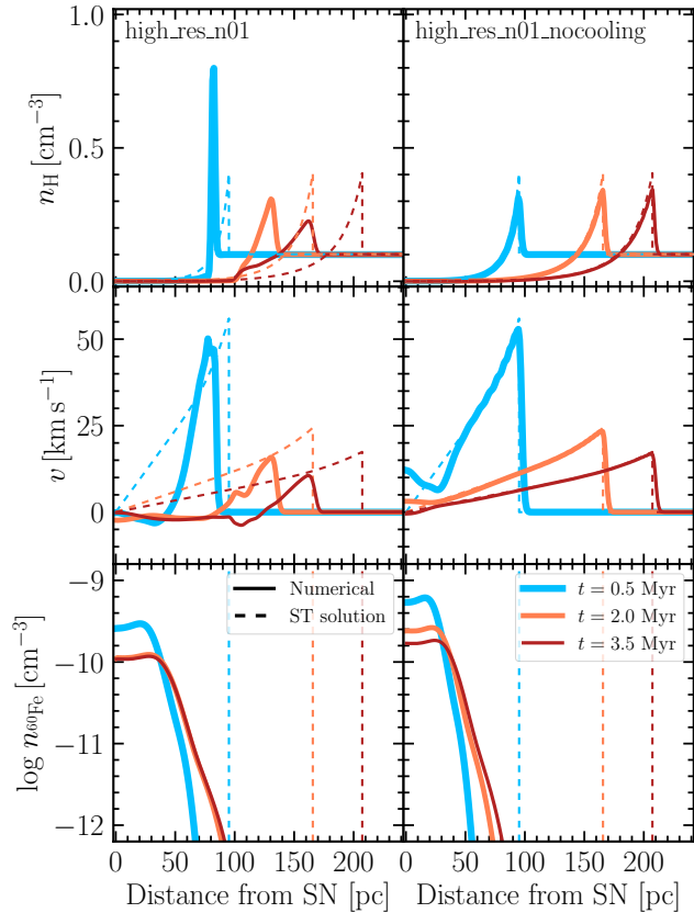
Figure 4. The average radial profiles of gas density ( top ), radial velocity ( middle ), and density of ^{60}\text{Fe} ( bottom ) in the simulations with ( high_res_n01 , left ) and without ( high_res_n01_nocooling , right ) gas radiative cooling. The profiles are shown at three consecutive times: 0.5 Myr (light-blue), 2.0 Myr (orange), and 3.5 Myr (dark-red). The mean ISM density is n_{\text{H}} = 0.1 \text{ cm}^{-3} in both runs. The width of radial bins is 1 pc. For reference, the dashed lines show the ST density profiles ( top ), ST velocity profiles ( middle ) and positions of the ST shock ( bottom ). To compute the ^{60}\text{Fe} -ejecta density we assumed a yield M_{60\text{Fe,tot}} = 10^{-4} M_{\odot} and no radioactive decay. The profiles in the run without radiative cooling agree with the ST solution at all times. The ejecta always lag behind the shock front and is always concentrated within a bubble of 100 pc.
