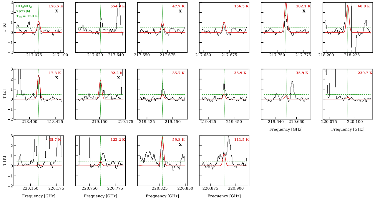
Fig. D.5: Showing that excitation temperature of 150 K does not match the observations for CH 3 NH 2 in source 767784. The various symbols are the same as Fig. 2. Again here some lines are overestimated and if the column density is decreased the lines that are perfect fits now will be underestimated.
