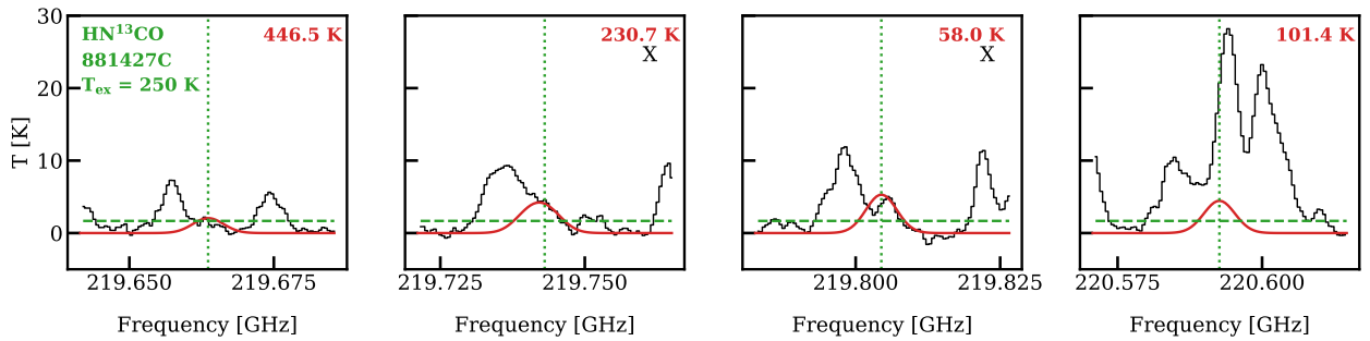
Fig. D.6: Best model for HN 13 CO of source 881427 (red) on top of the data (black). In this figure only lines with A_{ij} > 10^{-6} \text{ s}^{-1} and E_{\text{up}} < 700 \text{ K} are shown. Moreover, only one representative plot of the hyper fine structure of this molecule is shown to avoid repetition. The detected lines that are mainly considered for the fits are marked with an ‘X’ on the top right. The dashed lines shows the 3\sigma line.
