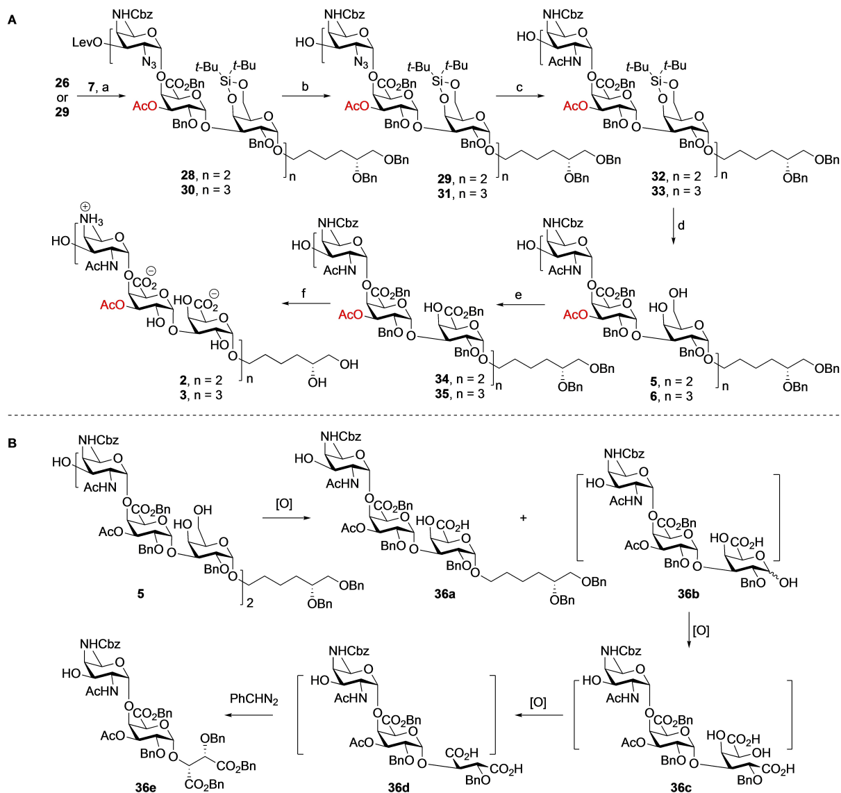
Scheme 3. A) Assembly of targets 2 and 3 . B) Oxidative cleavage leading to fragmentation of the oligosaccharides. Reagents and conditions: a) TBSOTf, DCM, 5Å MS, 0°C, 28 , 83%; 30 , 85%; b) N 2 H 4 ·H 2 O, pyridine, AcOH, 0°C→RT, 29 , 94%; 31 , 89%; c) i, PPh 3 , pyridine, H 2 O, THF, 70°C, 7 h; ii, Ac 2 O, NaHCO 3 , THF, H 2 O, 32 , 88%; 33 , 99%; d) HF·Py, THF, pyridine, 0°C, 5 , 92%; 6 , 96%; e) i, TEMPO, BAIB, t -BuOH, H 2 O, NaHCO 3 , EtOAc or MeCN, 4°C, 1 day; ii, PhCHN 2 , DCM, 34 , 58%; 35 , 66% (over two steps); f) Pd(OH) 2 /C, H 2 , t -BuOH, 0.1% AcOH in H 2 O, 3 days, 2 , 91%; 3 , 90%.
