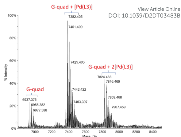
Figure 6 – Deconvoluted ESI mass spectrum of 10^{-6} M G4 incubated for 24 h with [\text{Pd}(\text{L}3)](\text{OAc})_2 in 100 mM ammonium acetate solution (pH 7.0) and in the presence of 60% EtOH. 3:1 metal complex/G4 molar ratio. The distribution of the ammonium ions has been omitted for clarity.
