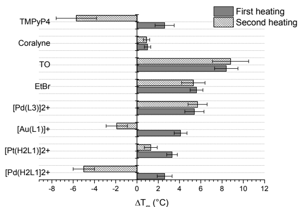
Figure 9 – Melting temperature difference ( \Delta T_m , °C) between that of a drug/RNA-4WJ mixture and that of the RNA-4WJ alone; C_{\text{drug}} = 2.0 \times 10^{-5} M, C_{\text{RNA4WJ}} = 1.0 \times 10^{-5} M, \text{CaCl}_2 182 \mu\text{M} , pH 7.0.
