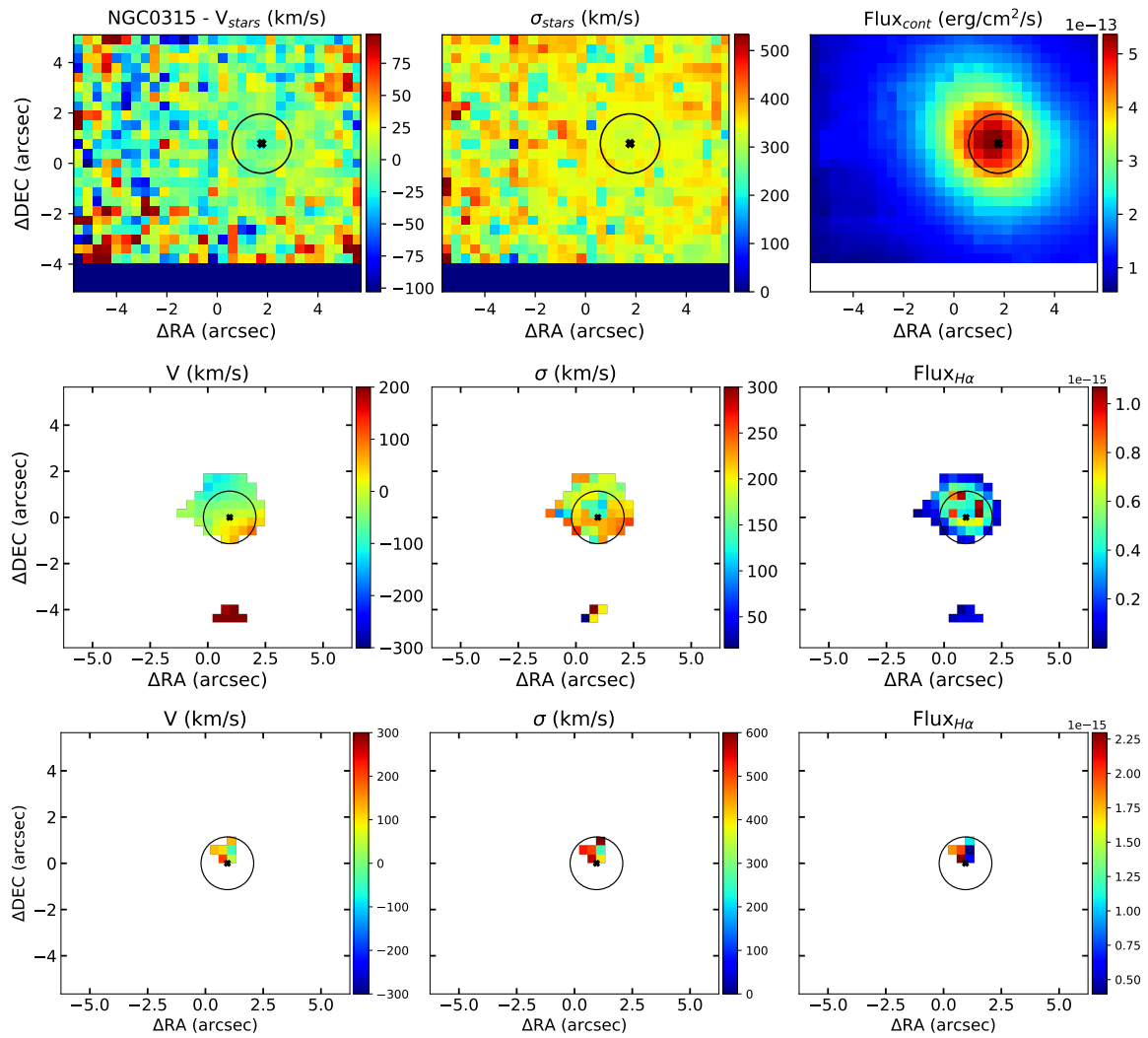
Fig. 5.5 Kinematic maps for the stellar (top panel) and ionised gas components of NGC 0315. The spectra of this galaxy was modelled with a narrow (second panel) and a secondary, unresolved (third panel) kinematical components per emission lines. Full description in 5.4.
