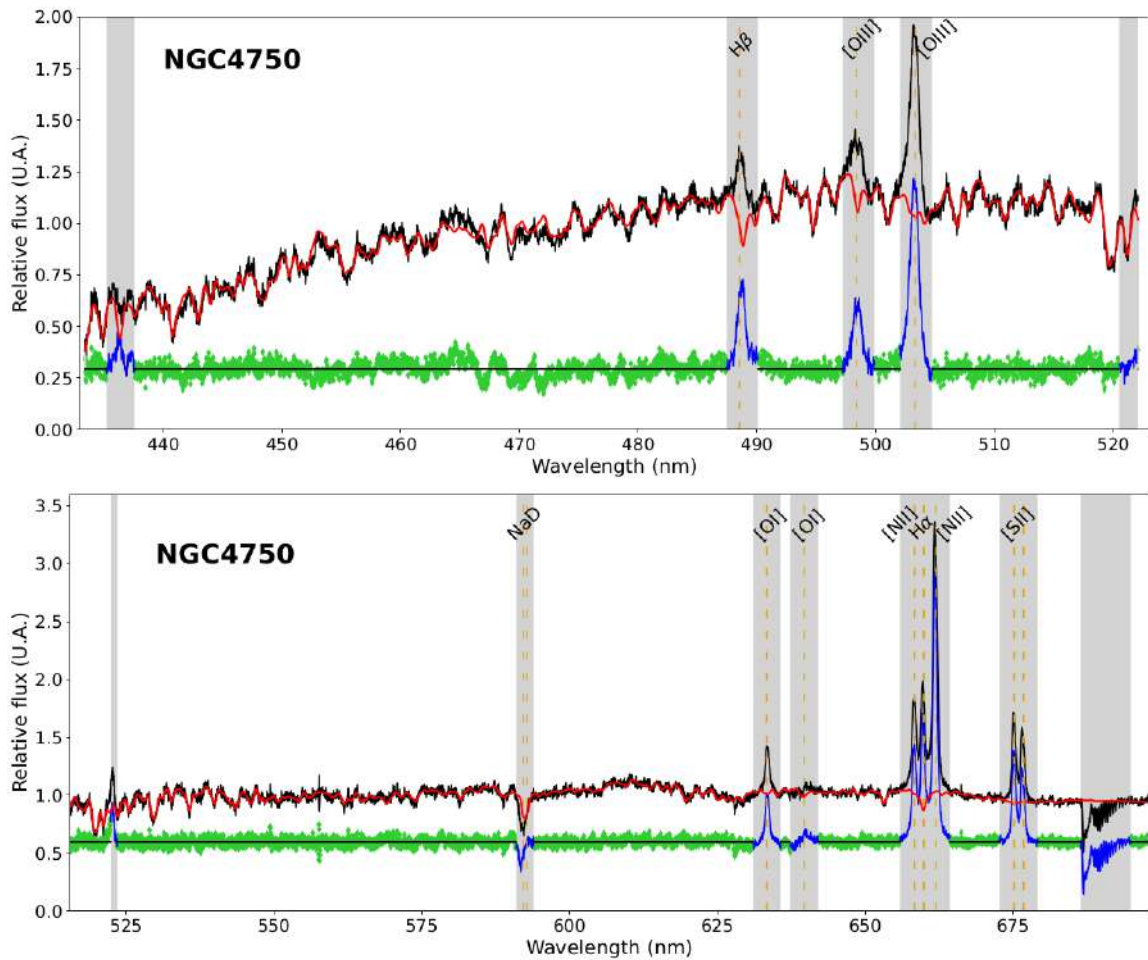
Fig. 5.2 Examples of the stellar modelling of the LR-B (top) and LR-V+LR-R (bottom) spectra extracted at the photometric centre of NGC 4750. In both panels: the red line shows the best fitting using \text{pPXF} , the green line shows the residuals of the fit, and the blue line is the final subtracted spectrum. The main emission and absorption lines are indicated with dashed vertical lines. Grey regions have been masked during the fitting.
