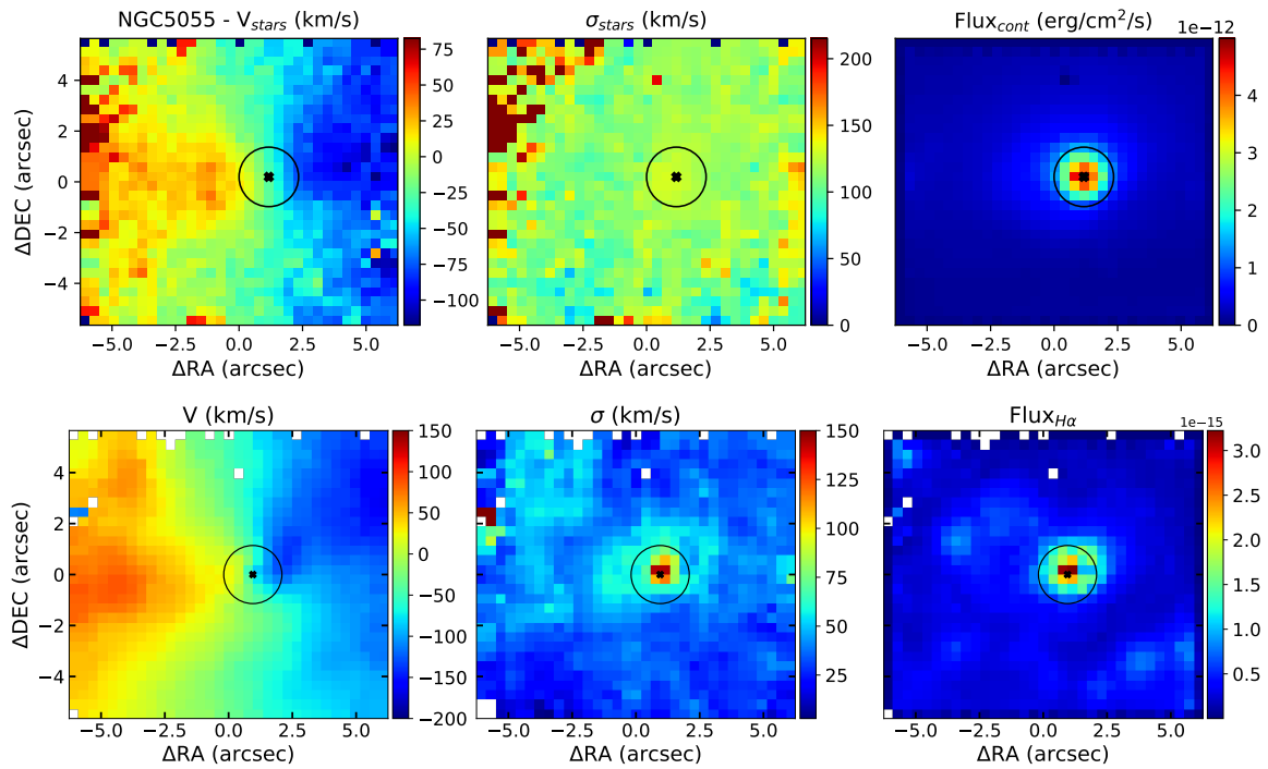
Fig. 5.10 Kinematic maps for the stellar (top panel) and ionised gas (bottom panel) components of NGC 5055. The spectra of this galaxy was modelled with a single narrow component on the emission lines. Full description in 5.4.
