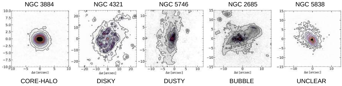
Fig. 3.3 Examples of the five proposed morphological classifications of the nuclear H \alpha emission (see Sect. 3.4). The complete images are in Appendix B.2.
