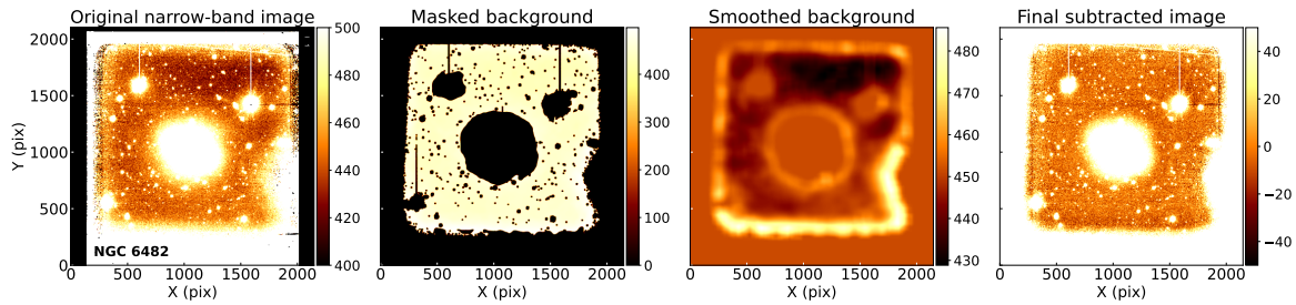
Fig. 3.2 Example of the background subtraction process for NGC 6482. Left: Original narrow-band image of the galaxy. Middle-left: Mask applied to the original image over imposed to the estimated background. Middle-right: Final smoothed background. Right: Final narrow-band image with the corresponding background subtracted. The scale on the left and right panels is around the background level to appreciate the differences before and after the subtraction. See Sect. 3.3 for more details.
