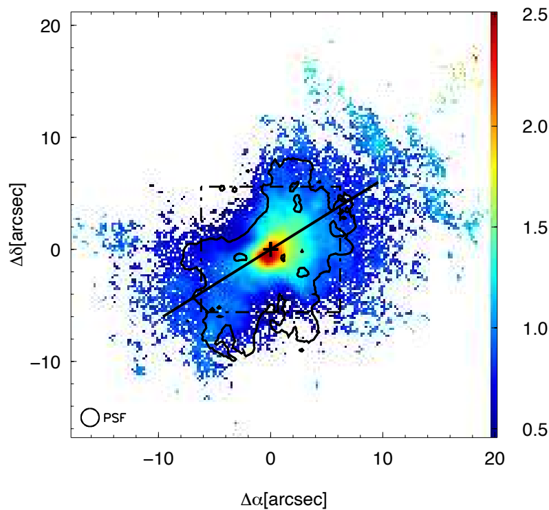
Fig. 4.8 NaD EW map (in \text{\AA} ) from MUSE cube. The dot-dashed square indicates the MEGARA field of view. The black solid line indicates the major axis of the stellar rotation (Table 4.2). The contours indicate the region with enhancement velocity dispersion of emission lines (see Sect. 4.4.2 and e.g. Fig. 4.5).
