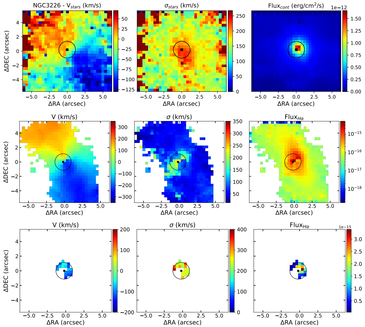
Fig. 5.6 Kinematic maps for the stellar (top panel) and ionised gas components of NGC 3226. The spectra of this galaxy was modelled with a narrow (second panel) and a secondary (third panel) kinematical components per emission lines. Full description in 5.4.
