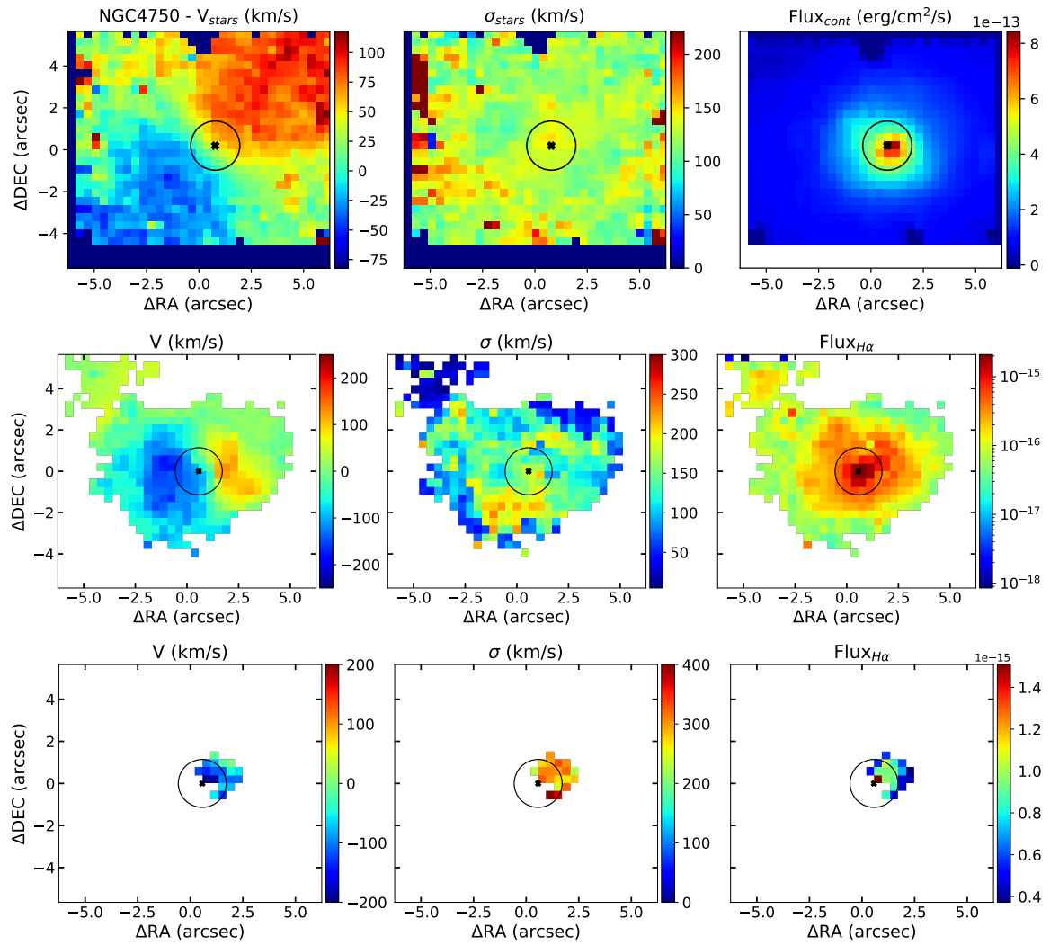
Fig. 5.9 Kinematic maps for the stellar (top panel) and ionised gas components of NGC 4750. The spectra of this galaxy was modelled with a narrow (second panel) and a secondary (third panel) kinematical components per emission line plus a broad component under H \alpha . Full description in 5.4.
