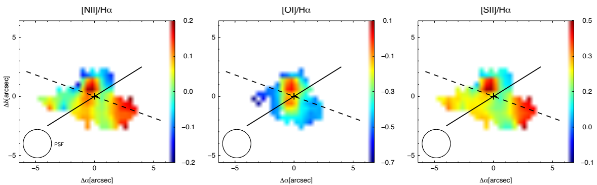
Fig. C.18 As in Fig. C.17, but for the second component. The long-dashed line gives the PA of the 20 cm emission (Table 4.1), as in Fig. C.7.
