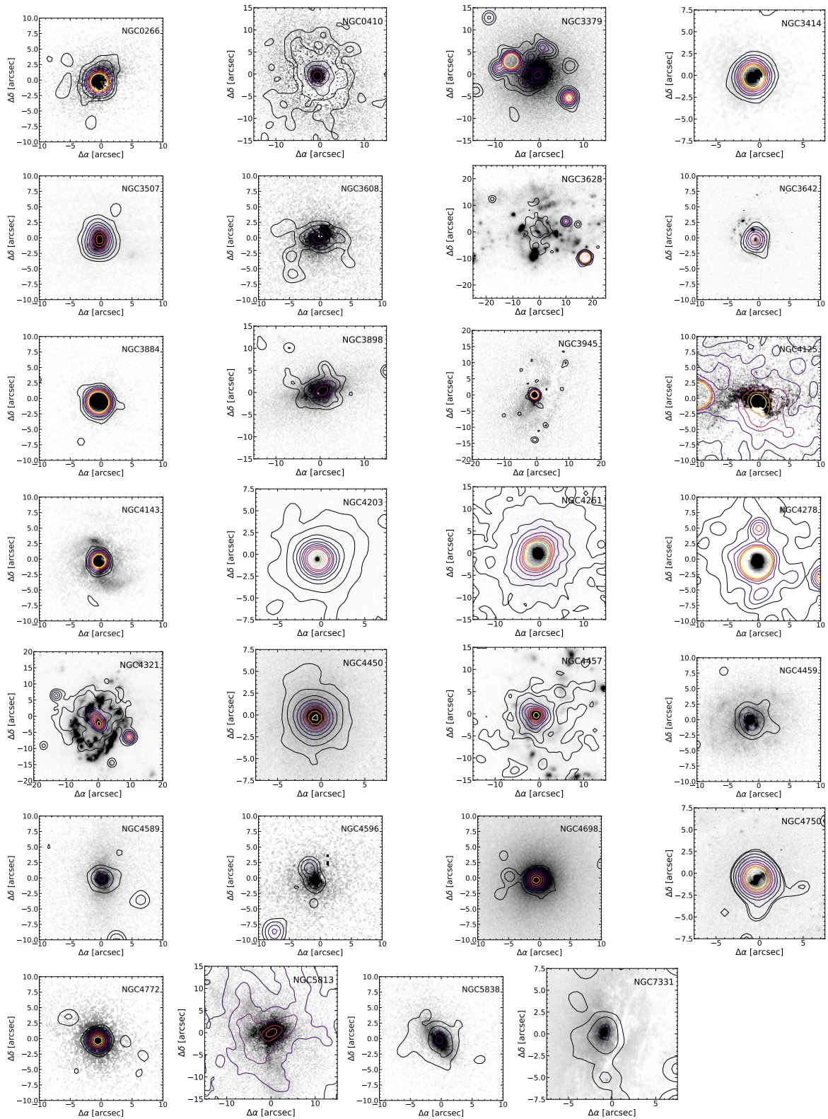
Fig. 3.5 H\alpha images with overlaid contours of the X-ray emission from Chandra. The contour levels are at 3\sigma (black), 7\sigma (black), 15\sigma (black), 25\sigma (dark-purple), 40\sigma (purple), 60\sigma (light-purple), 80\sigma (red), 100\sigma (orange) and 150\sigma (yellow).
