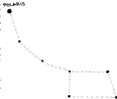
URSA MINOR
