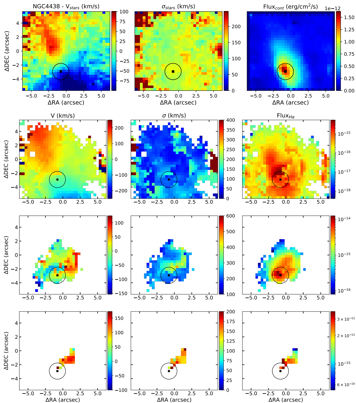
Fig. 5.12 Kinematic maps for the stellar (top panel) and ionised gas components. The spectra of this galaxy was modelled with a primary (second panel), a secondary (third panel) and a third (bottom panel) kinematical components per emission line. Full description in 5.4.
