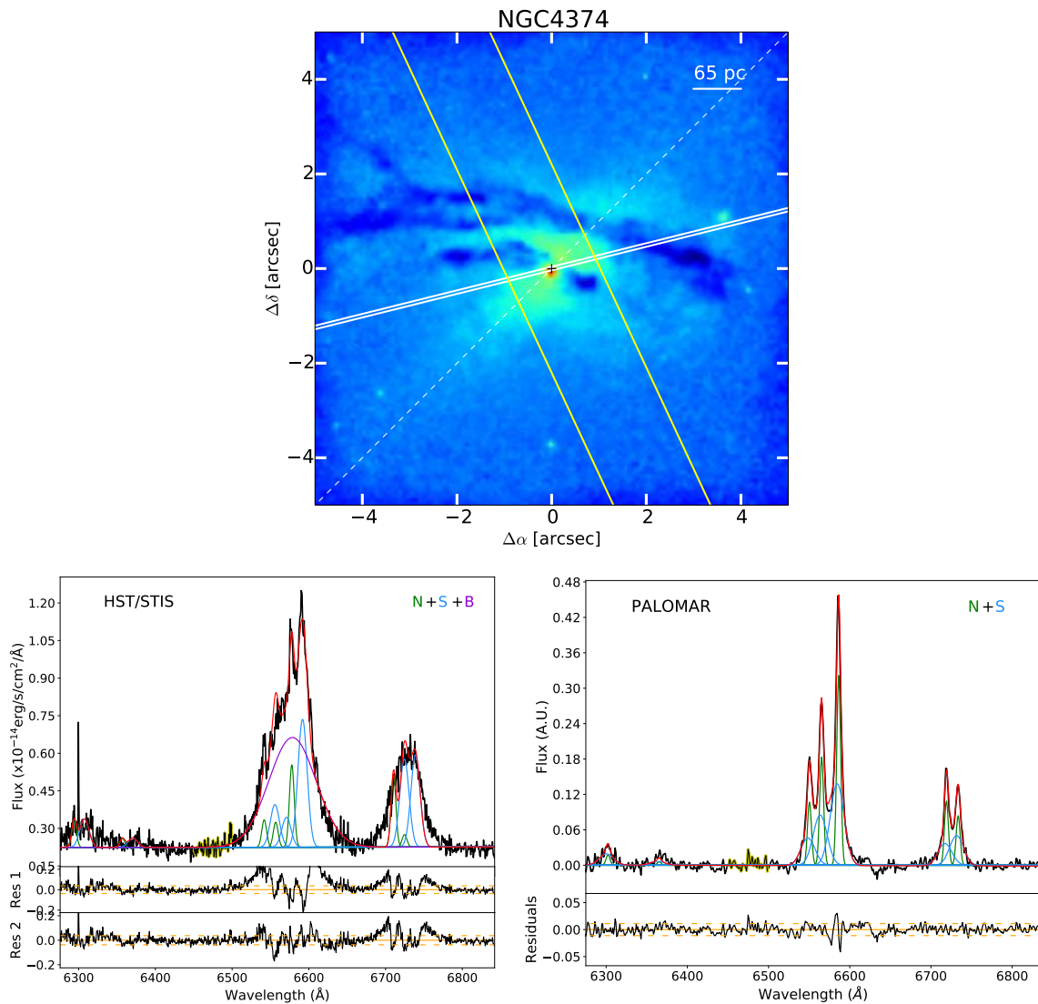
Fig. A.11 (General description in Appendix A.2). NGC 4374: In the HST/STIS spectrum, [S II] lines are severely blended, and only the [O I] \lambda 6300Å line is visible (with low S/N). This complicated the modeling for the other lines, so the fit was performed considering the narrow peaks of [N II]-H \alpha blend (see Sect. 2.3), which results in high residuals under the [S II] lines. A broad component is needed in this decomposition. For the Palomar spectrum, all the emission lines are well-modeled with two Gaussian components.
