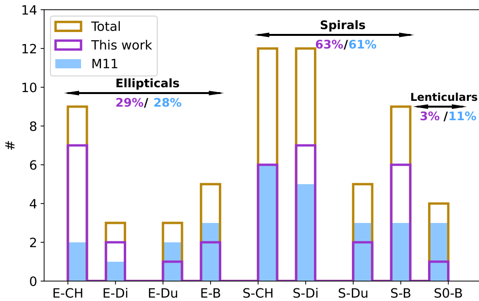
Fig. 3.7 Histogram of the morphological type of the host galaxy and the classification of the nuclear H\alpha emission. It is divided into ellipticals (E), spirals (S) and lenticulars (S0); ‘CH’ stands for ‘Core-halo’, ‘Di’ for ‘Disky’, ‘Du’ for ‘Dusty’ and ‘B’ for ‘Bubble’. Purple lines indicates the sample from this work; blue for M11; and yellow is the combination of both samples. We have not included unclear cases or irregular galaxies in the figure, and thus the percentages do not sum up 100%.
