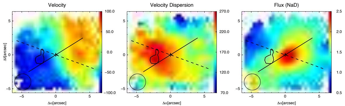
Fig. 4.10 Neutral gas velocity field ( \text{km s}^{-1} ), velocity dispersion ( \text{km s}^{-1} ), and flux intensity (mJy) maps for the single kinematic component used to model NaD. The black lines are as in Fig. C.13. Specifically, the black solid line indicates the major axis of the stellar rotation (Table 4.2). The dashed lines indicate the orientation of the radio jet (Table 4.1). The contours indicate the region at high velocity dispersion (Sect. 4.5.4 for details).
