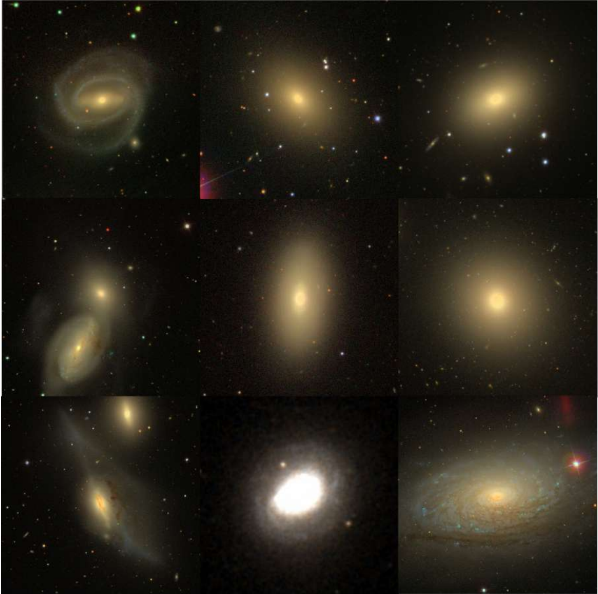
Fig. 5.1 Optical images of the nine LINERs observed with MEGARA. From left to right, up to down: NGC 0266, NGC 0315, NGC 1052, NGC 3226, NGC 3245, NGC 4278, NGC 4438, NGC 4750 and NGC 5055. All images have been obtained from the Sloan Digital Sky Survey DR9, except for NGC 4750, that is from the Digitalized Sky Survey. In all images, north-east is up-left.
