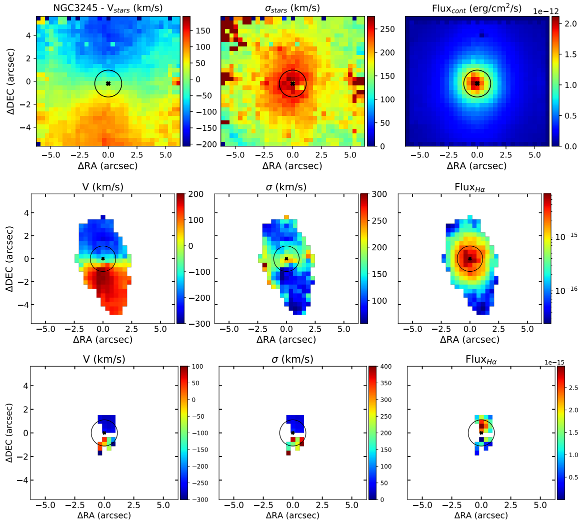
Fig. 5.7 Kinematic maps for the stellar (top panel) and ionised gas components of NGC 3245. The spectra of this galaxy was modelled with a narrow (second panel) and a secondary (third panel) kinematical components per emission lines. Full description in 5.4.
