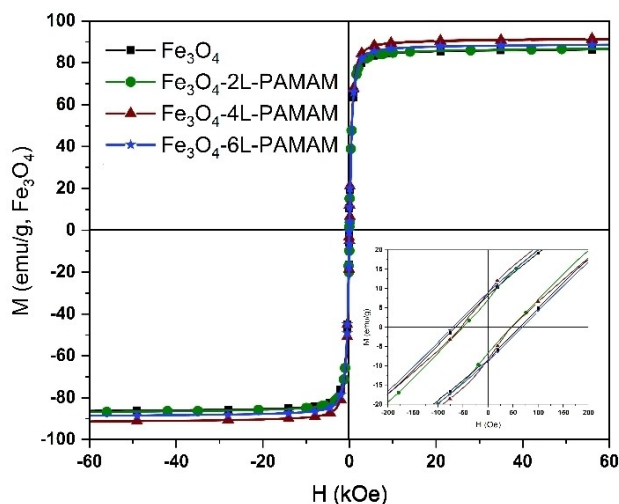
Figure 10. Magnetization hysteresis loop measured at 300 K for the \text{Fe}_3\text{O}_4 nanoparticles and the corresponding \text{Fe}_3\text{O}_4 @LbL-PAH-PAA-PAMAM- \text{NH}_2 composite materials containing 2, 4, and 6 layers of polyelectrolyte ( M = magnetization and H = magnetic field strength).
