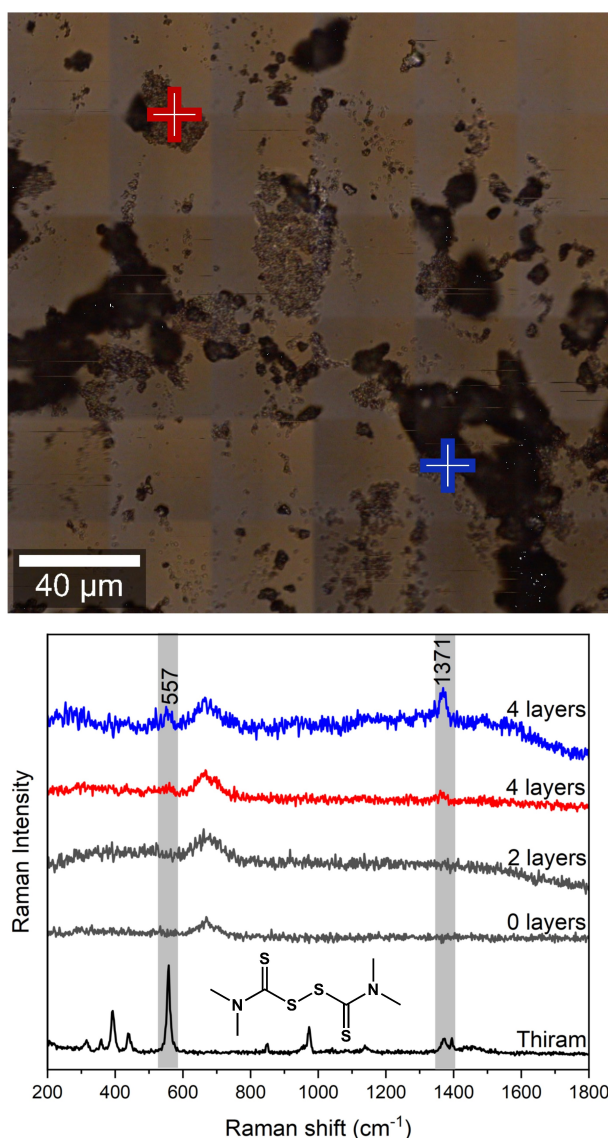
Figure 14. Preliminary SERS experiments using \text{Fe}_3\text{O}_4@ LbL-PAH/PAA-PA-MAM-AuNPs to probe thiram at 100\ \mu\text{M} . Top: Optical microscopy image of the magneto plasmonic substrate with 4 layers of PAH/PAA and bottom: the corresponding SERS spectra at the marked points. The Raman spectrum of thiram powder and the typical SERS spectra of the magneto-plasmonic with 0 and 2 layers are presented for comparative purposes.
