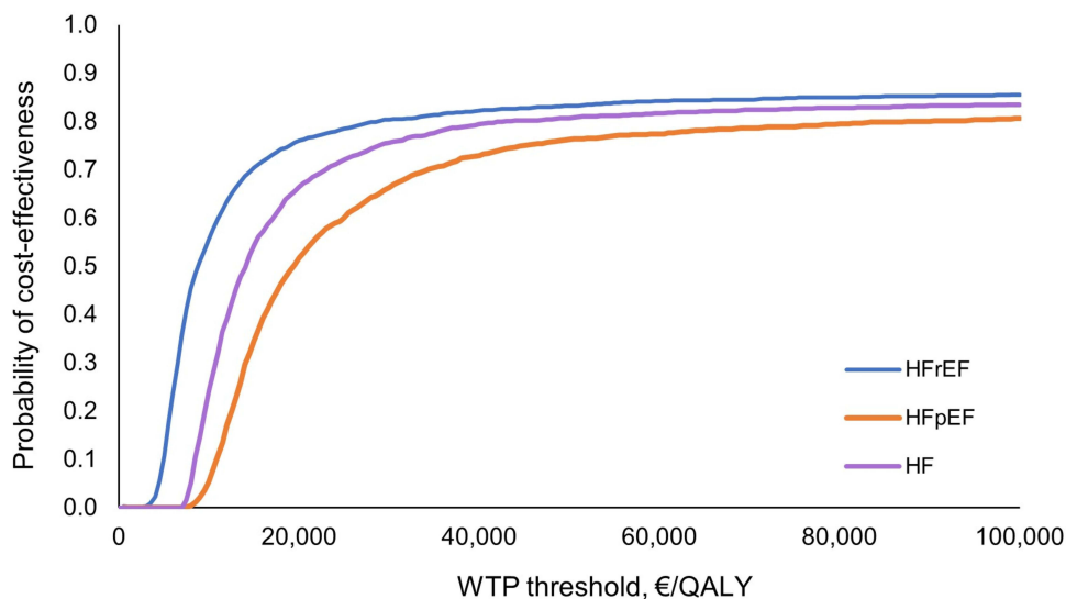
Figure 3 The cost-effectiveness acceptability curve for empagliflozin + SC versus placebo + SC in HF, HFrEF and HFpEF population. Abbreviations: SC, standard care; HF, heart failure; HFrEF, heart failure with reduced ejection fraction; HFpEF, heart failure with preserved ejection fraction.
