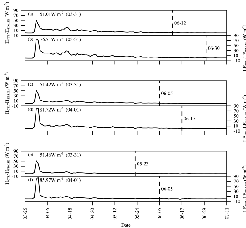
Figure 8. The difference in the daily average sensible and latent heat between the CTL and the three sensitivity simulations under the water temperature profiles in SIM_E1, SIM_E2, and SIM_E3.
