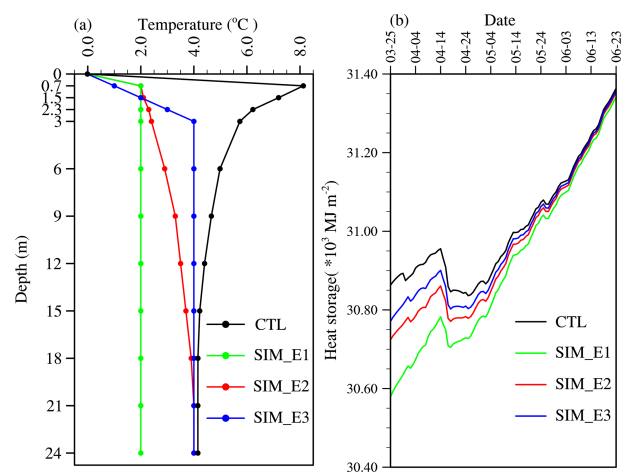
Figure 7. (a) The initial water temperature profiles in the model are set on 25 March 2016, and the corresponding daily average (b) lake heat storage is simulated. SIM_E1 , SIM_E2 , and SIM_E3 are three different sensitivity simulations.
