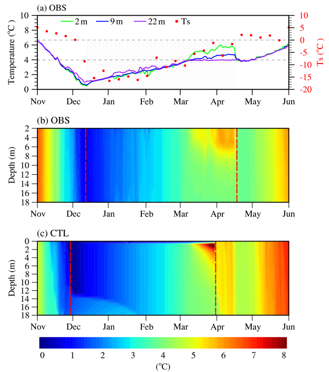
Figure 2. (a) The daily average water temperature observations of Ngoring Lake at the surface ( T_s ) and at 2, 9, and 22 m from 1 November 2015 to 1 June 2016. T_s is MODIS lake surface temperature. The gray reference lines denote 3.98 and 0 \text{ }^\circ\text{C} , respectively. The shaded pink area denotes the ice-covered period. The water temperature profile (b) observed and (c) simulated in CTL. The ice-covered period is represented between the two dashed red lines.
