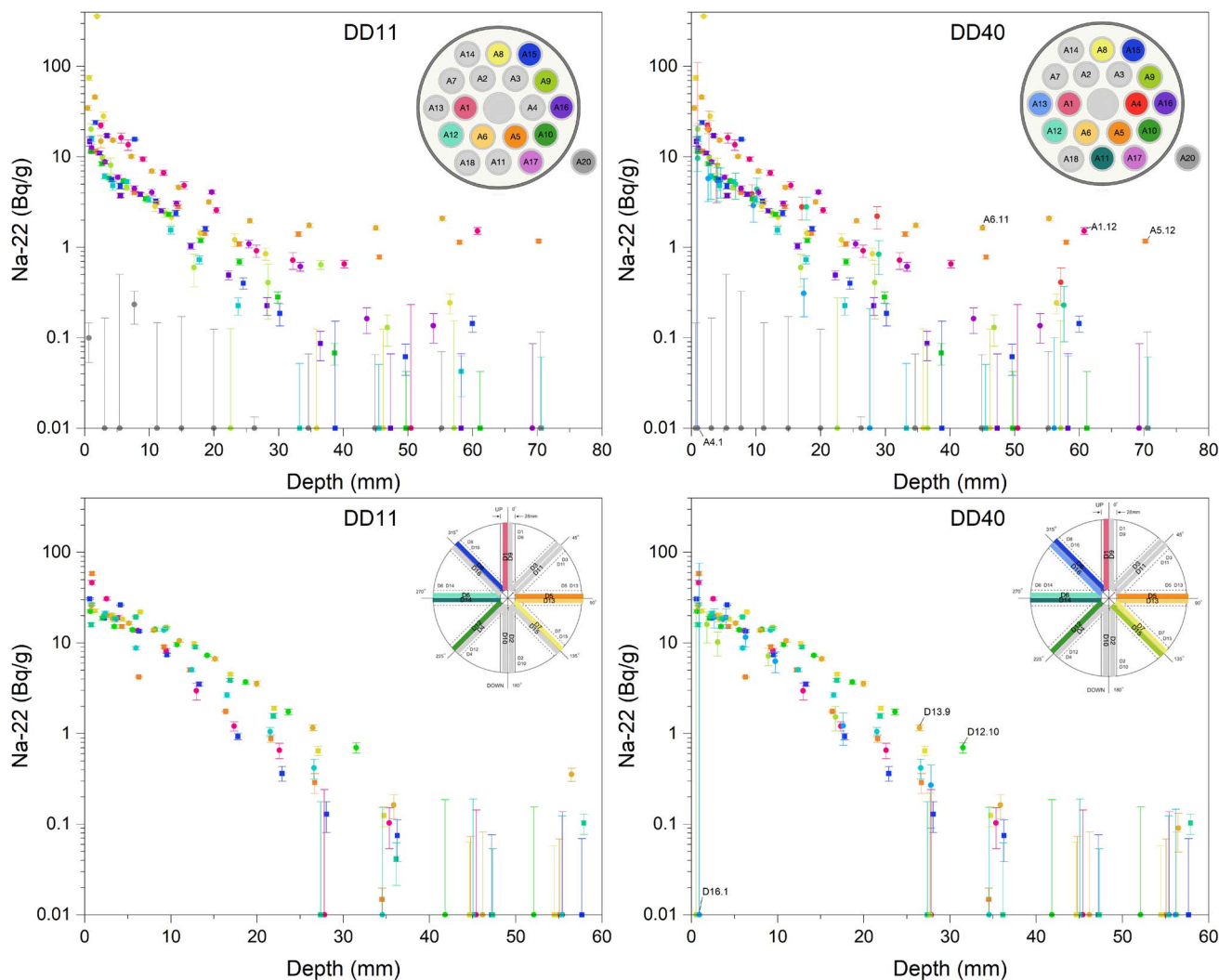
Figure 1. Na-22 activity in A and D cores in DD11 and DD40. Data points below detection limit are plotted on the bottom axis of the plots.
