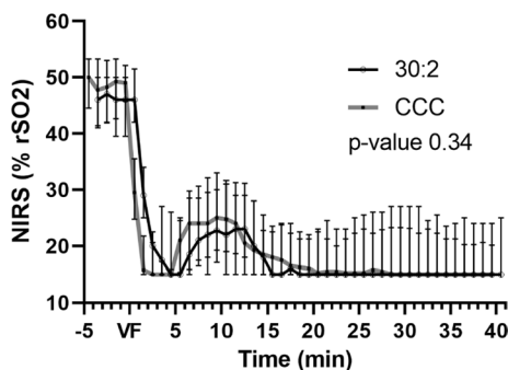
Fig. 5 NIRS values during experimental cardiopulmonary resuscitation shown as medians and interquartile ranges. The p-value is given for a linear mixed model between the groups. NIRS: near-infrared spectroscopy; rSO 2 : regional oxygen saturation index; VF: ventricular fibrillation; CCC: continuous chest compressions
