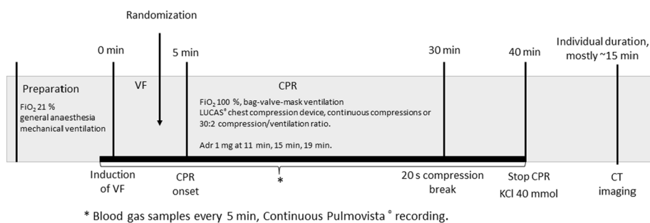
Fig. 1 Timeline of the experimental protocol. Adr: adrenaline; \text{FiO}_2 : fraction of inhaled oxygen; VF: ventricular fibrillation; CPR: cardiopulmonary resuscitation; KCl: potassium chloride; CT: computed tomography
