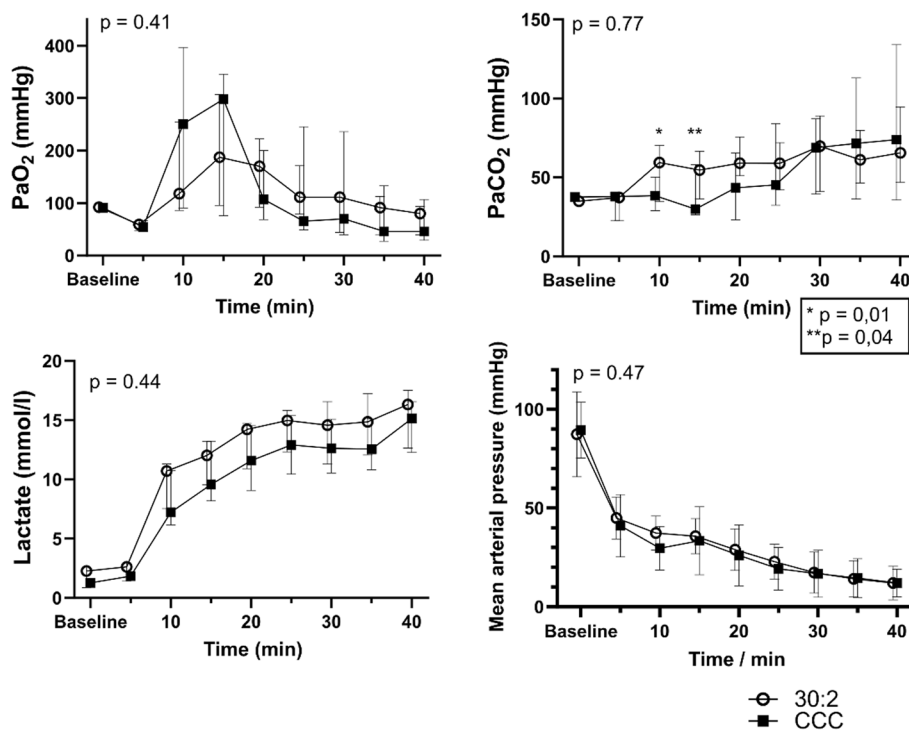
Fig. 3 Arterial oxygen pressures (PaO 2 ), carbon dioxide pressures (PaCO 2 ), lactate levels and mean arterial pressures during experimental cardiopulmonary resuscitation shown as medians and interquartile ranges. The p-value is given for a linear mixed model between the groups. CCC: continuous chest compressions
