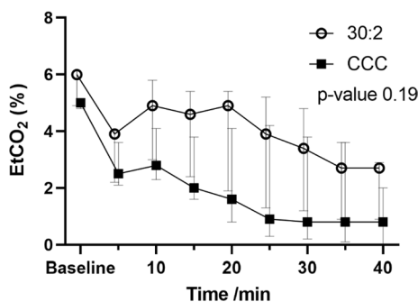
Fig. 4 EtCO 2 levels of the 30:2 and CCC groups during experimental cardiopulmonary resuscitation shown as medians and interquartile ranges. The p-value is given for a linear mixed model between the groups. EtCO 2 : end-tidal carbon dioxide; CCC: continuous chest compressions
