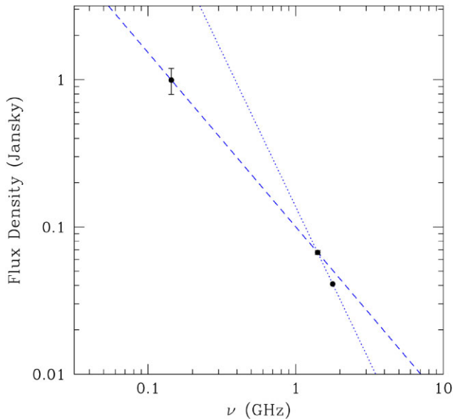
Figure 4. Flux density of the diffuse emission in A523 versus frequency. The power-law fit of the 144 MHz and 1.410 GHz data points is shown in dashed blue, while the fit of the 1.410 GHz and 1.782 GHz data points in dotted blue.
