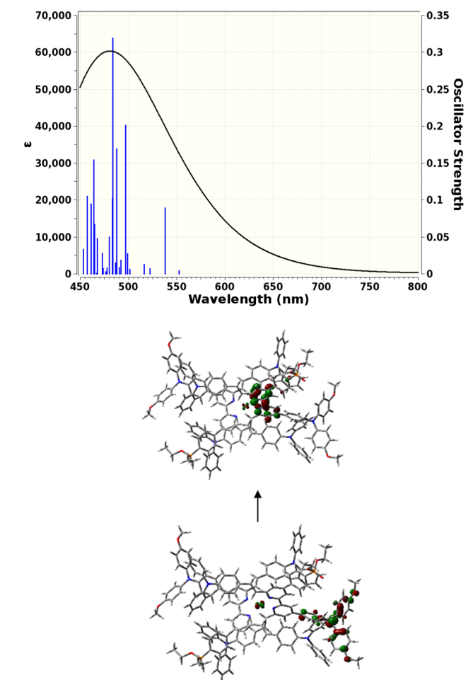
Fig. 8 Top: TD-DFT-simulated UV-visible absorption spectrum of [\text{Cu}(\mathbf{6e})_2]^+ . Black curve: estimated lineshape including broadening. Blue lines: calculated singlet transitions with corresponding oscillator strengths. Bottom: 0.05 a.u. isocontour surfaces of NTOs that describe the [\text{Cu}(\mathbf{6e})_2]^+ electronic transition at 538 nm. One donor orbital (bottom) and one symmetry-equivalent acceptor orbitals (top) adequately describe the transition density with coefficient 0.94.
