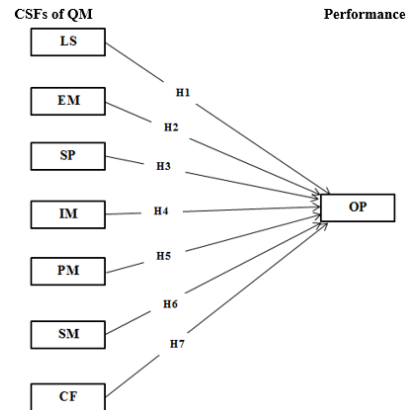
Figure 1. Study Framework
