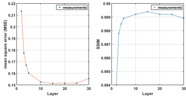
Figure 7: Calculated MSE and SSIM of the LD model at different layers.
