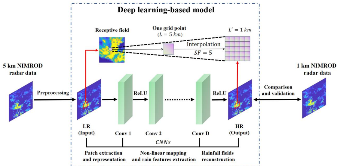
Figure 4: Overview of the proposed approach. The left part is the raw data provided by NIMROD radar. The middle part (dashed box) is the deep learning-based rain model. As the soul of the whole model design, it uses the CNNs to grasp the underlying rain properties and the non-linear mapping relationship between low resolution (LR) rain map and the high one, so the high resolution (HR) point rainfall rate can be accurately estimated. Note that the extent that resolution is improved is dependent on the value of SF. For example, here we set the SF=5 so the space resolution will be improved 5 times. The right part is the 1 \text{ km} NIMROD data used for model comparison and validation.
