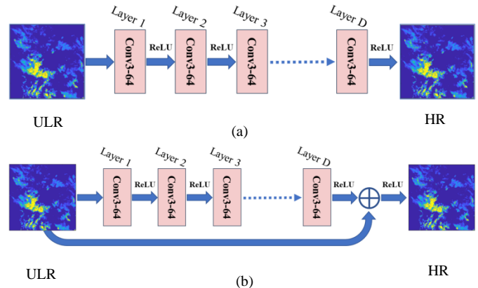
Figure 5: Network structure, (a) is LI model, and (b) is LD model. A series of layers (convolutional and non-linear) have been cascaded repeatedly in the network. The input (ULR NIMROD radar data) goes through layer-by-layer and transforms into a high-resolution point rainfall rate. 64 filters for each convolutional layers and sample feature maps have been presented for visualization.
