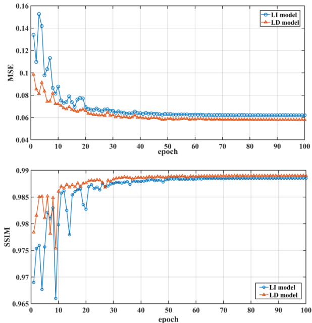
Figure 6: Plotting of the MSE and SSIM with changing epochs for the LI model and LD model.
