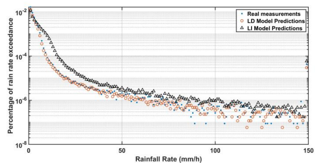
Figure 9: Complementary cumulative distribution function of rainfall rate at Portsmouth for one month period.
