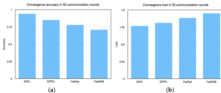
Figure 7. Convergence comparison of the proposed SHFL with state-of-the-art techniques, (a) comparison accuracy over MNIST; (b) comparison loss over MNIST.
