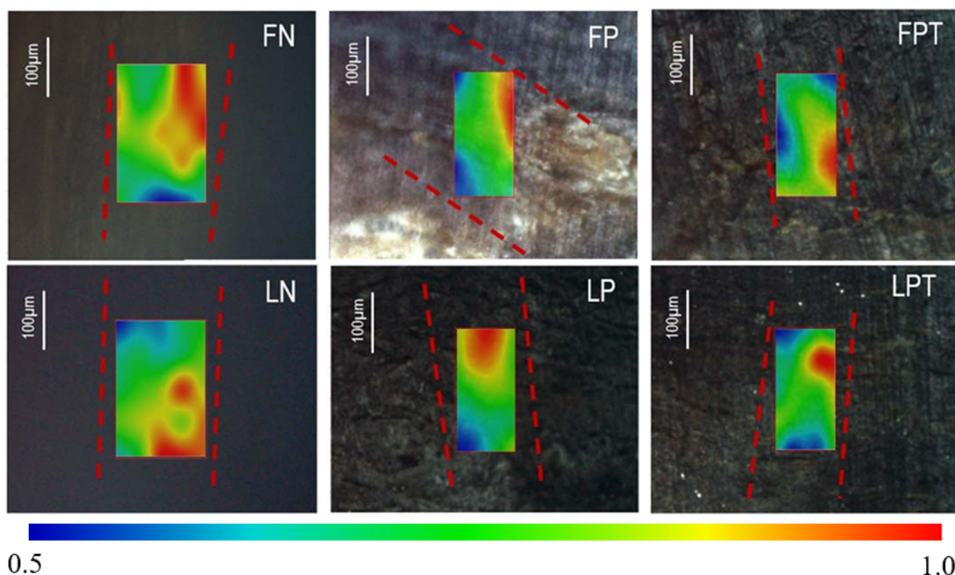
Figure 7. Infrared distribution on the samples surface band at 3500\text{ cm}^{-1} of fir wood before treatments (FN), after densification (FP) and after densification with TEOS (FPT) and larch wood before treatments (LN), after densification (LP) and after densification with TEOS (LPT); the contours of the analyzed fibers are highlighted with red dotted lines.
