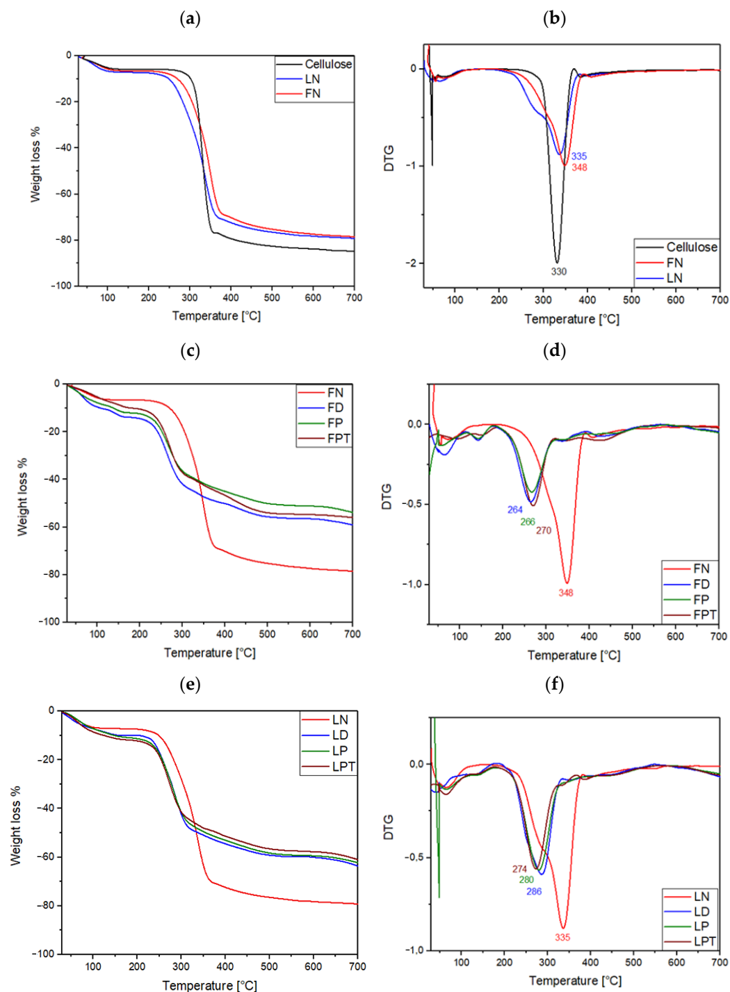
Figure 5. Comparison of the thermogravimetric profile of fir (FN) and larch (LN) woods with a cellulose sample (a) and their first derivatives (b); thermogravimetric profile of fir wood (c) before treatments (FN), after delignification process (FD), after densification (FP) and after densification with TEOS (FPT) and their first derivatives (d); thermogravimetric profile of larch wood I before treatments (LN), after delignification process (LD), after densification (LP) and after densification with TEOS (LPT) (e) and their first derivatives (f).
