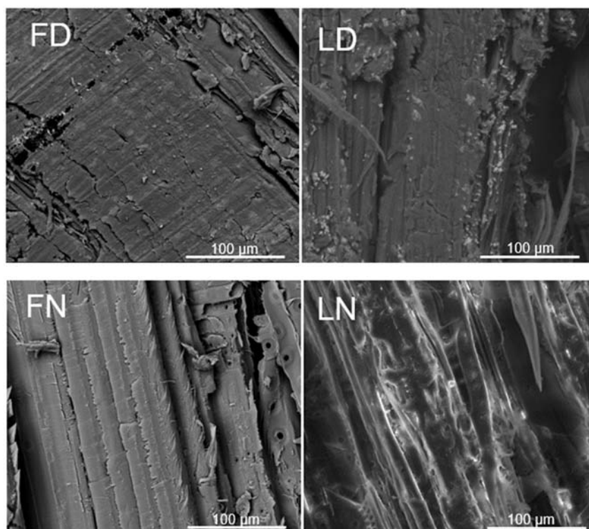
Figure 3. SEM images of fir and larch sample surfaces before (FN: Natural Fir; LN: Natural Larch) and after (FD: Delignified Fir; LD: Delignified Larch) the delignification process. All images were recorded at 1000× magnification.
