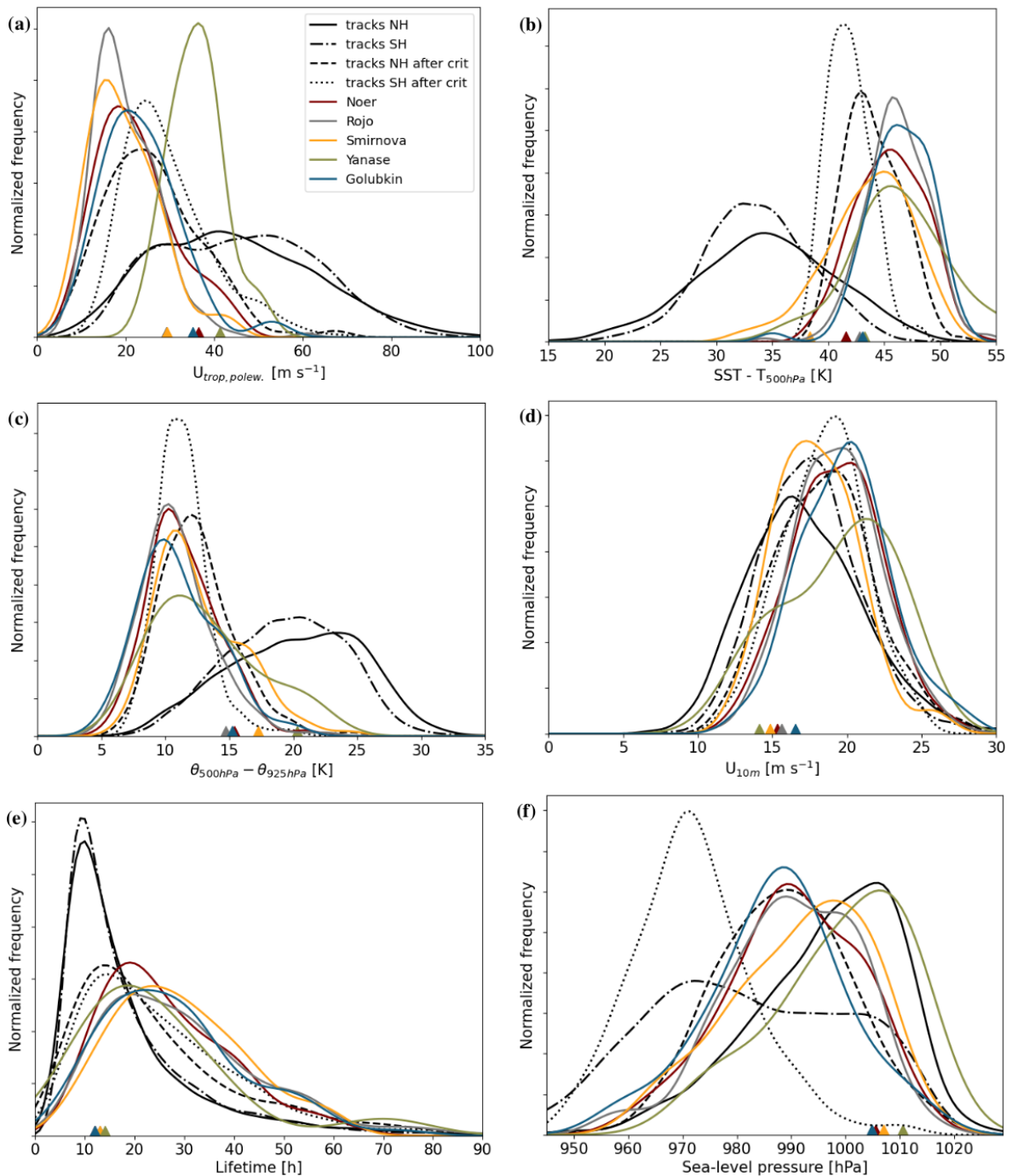
Figure 2. As Fig. 1. Parameter distributions for polar lows from the lists (colours) and cyclone tracks of the Northern Hemisphere and Southern Hemisphere (black). Cyclone tracks that remain after the application of the four polar-low criteria for the two hemispheres (black dotted and dashed) are displayed to demonstrate the quality of the polar-low criteria. (a) The maximum wind speed at the tropopause poleward of the system, U_{\text{trop.polew.}} , is computed as the lifetime mean of the track. (b) The temperature difference between the 500 hPa level and the sea surface, \text{SST} - T_{500\text{hPa}} , and (d) the maximum near-surface wind speed, U_{10\text{m}} , as the lifetime maximum. (c) The potential temperature difference between 500 and 925 hPa, \theta_{500\text{hPa}} - \theta_{925\text{hPa}} , and (f) the sea-level pressure, as the lifetime minimum. (e) The lifetime is the duration of the track.
