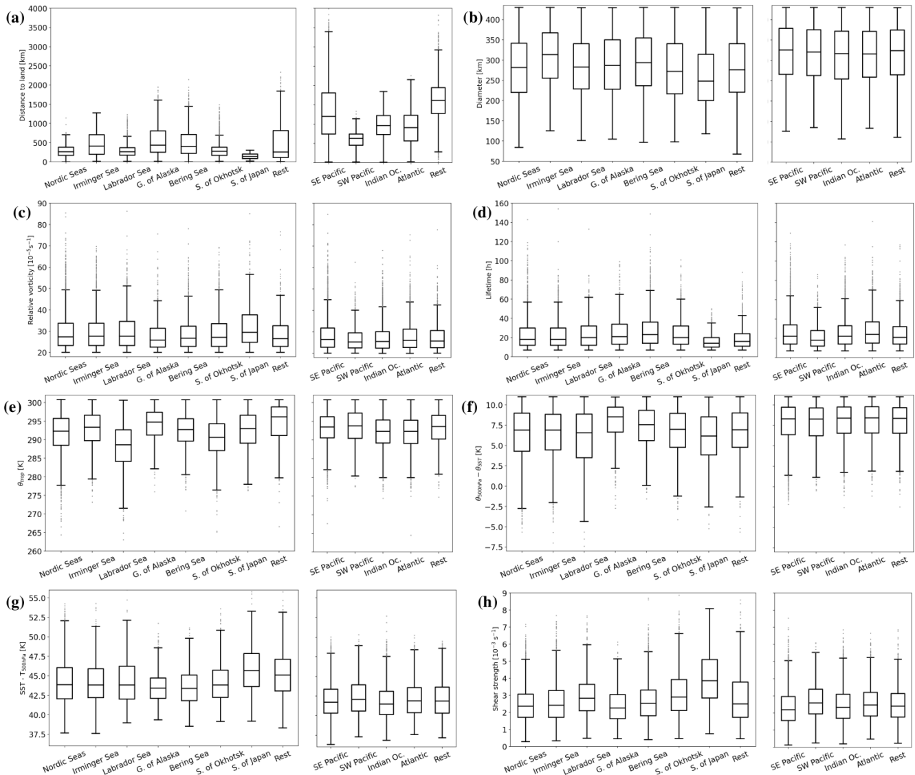
Figure 7. Parameter distributions of polar lows for the different regions. The lifetime maximum of the polar-low tracks is used for the computation of (a) the distance to land, (b) the vortex diameter, (c) the relative vorticity, (g) SST - T_{500\text{hPa}} , and (h) the shear strength. For (e) \theta_{\text{trop}} , the lifetime mean is calculated, and for (f) \theta_{500\text{hPa}} - \theta_{\text{SST}} , the lifetime minimum is calculated. (d) The lifetime is the duration of the polar low.
