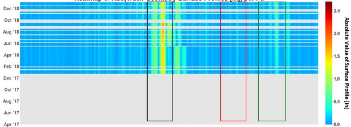
Line Plot of Track-Geometry Surface Profiles [in] per Ft.
