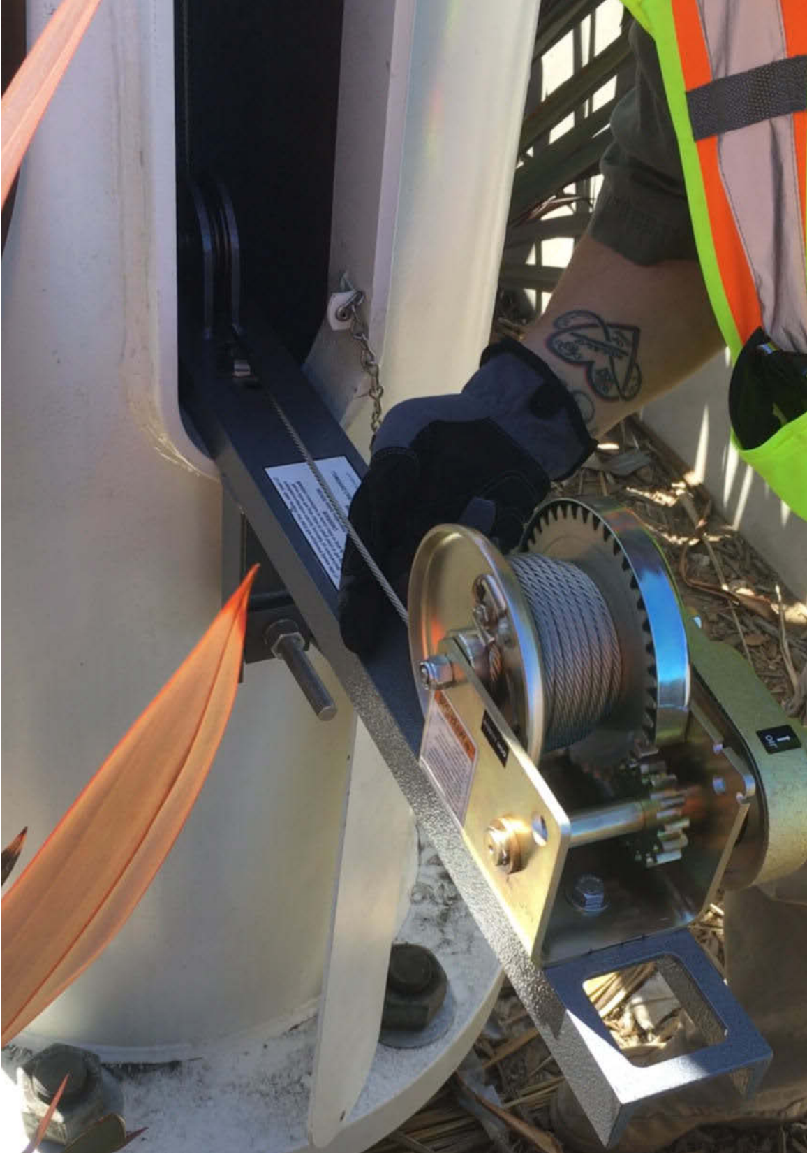
Figure 63. Hand Guiding Winch Cable
