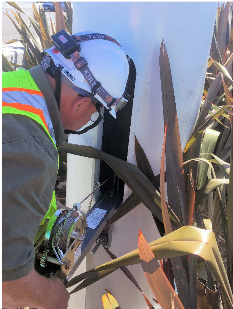
Figure 62. Attach Winch Tool
