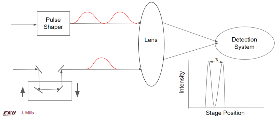
Figure 21: A diagram showing the setup of the probe pulse method for measuring the delay created by the AOM pulsed shaper.
