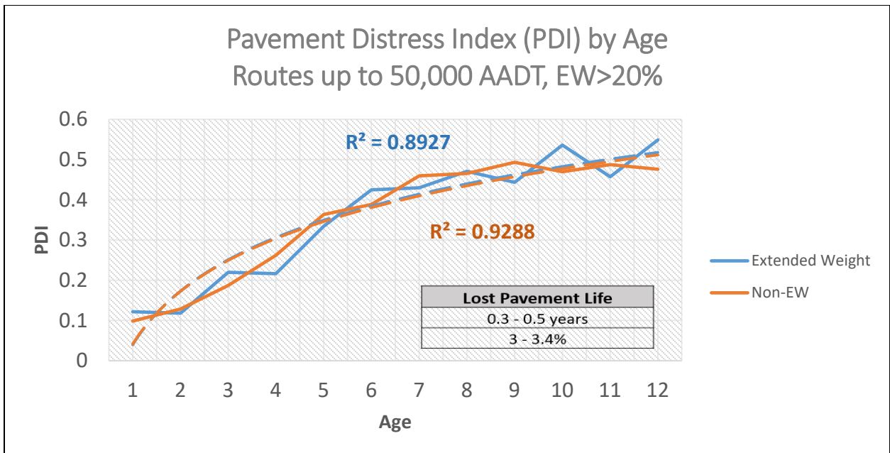
Figure 5.5 Pavement Distress Index (PDI) by Age (Routes up to 50,000 AADT, EW>20%)
