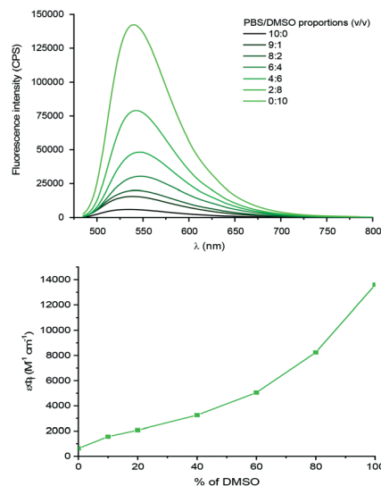
Fig. 1 Top panel: Evolution of the fluorescence intensity and lower panel: brightness ( \epsilon\Phi_f ) of solutions of Van-Green (5 \mu\text{M} ) with increasing percentages of DMSO in PBS upon excitation at 475 nm.
