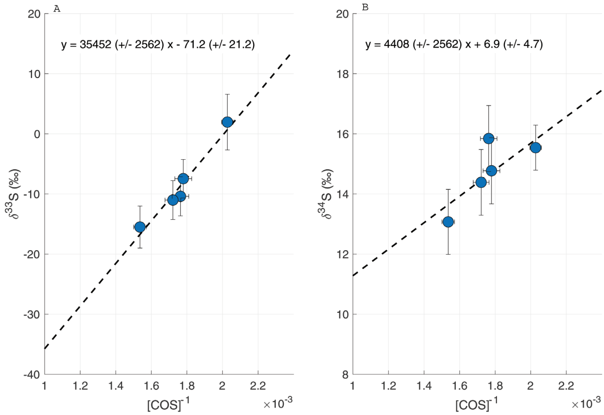
Figure 10. Keeling plot of the samples taken inside a highway tunnel, for \delta^{33}\text{S} (A) and \delta^{34}\text{S} (B).
