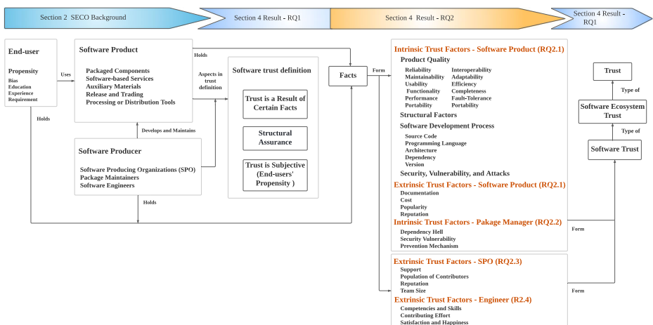
Fig. 1 This study outline provides the graphical overview of this work. Specifically, it provides an overview of the SECO background, along with the results of the two research questions. The sections that they correspond to in the study, as well as the research questions are provided at the top
