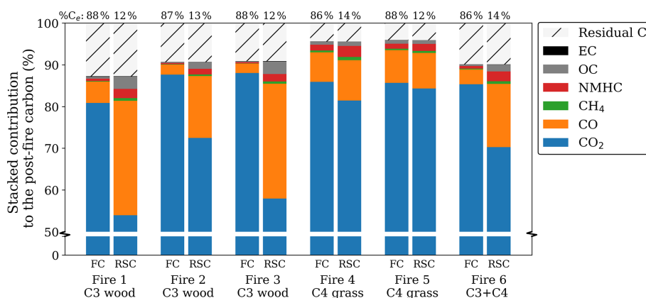
Figure 1. Post-fire partitioning of carbon for the flaming (left) and smouldering (right) phase for oak wood chips ( C_3 ) and prairie grass ( C_4 ). Note that the bottom 50%, containing only CO_2 , was cut from the graph to emphasize the smaller fractions. The numbers over the bars represent the percentage of carbon emitted in each phase. As the residue was only measured at the end of the fire, the residual carbon, calculated as the post-fire carbon in the residue over the pre-fire carbon in the fuel, was equally allocated to both phases. Carbon in NMHC was estimated to be 3.5 times the carbon in CH_4 based on Andrea (2019).
