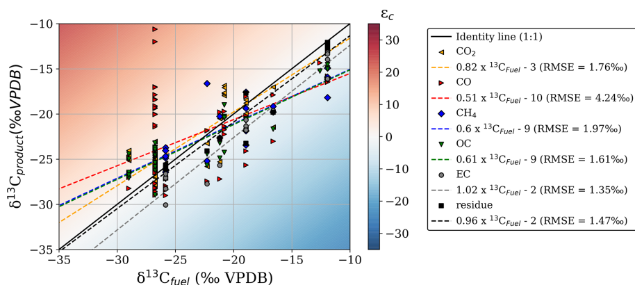
Figure 2. \delta^{13}C of the combustion products compared to the \delta^{13}C of the original fuel. The plot area colour scale represents the absolute fractionation ( \epsilon ) compared to the precursor fuel. Linear regression formulas of the different curves and RMSE values are given in the legend on the right.
